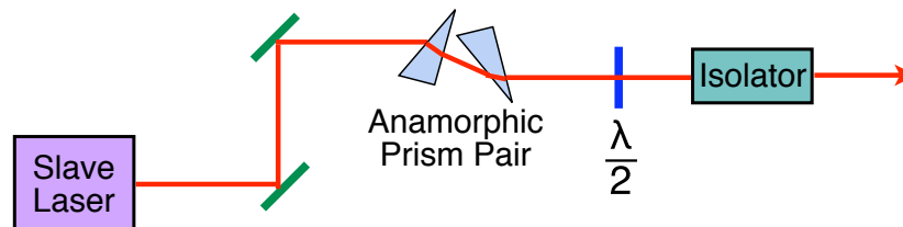
Figure 2.2. Schematic of the optical elements used to control and shape the diode laser's output beam, including the steering mirrors, anamorphic prism pair, half-wave plate, and optical isolator.
