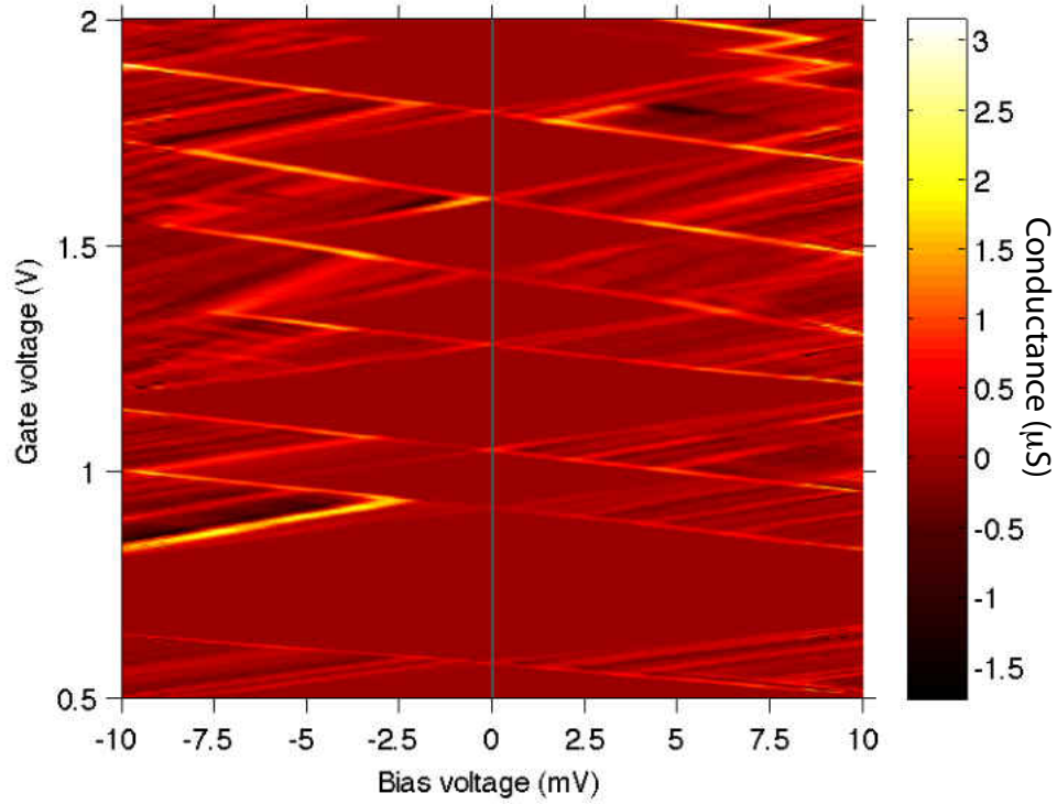
Figure 2.3. Coulomb blockade diamond of differential conductance as a function of bias and gate voltages measured at T = 550 mK.
