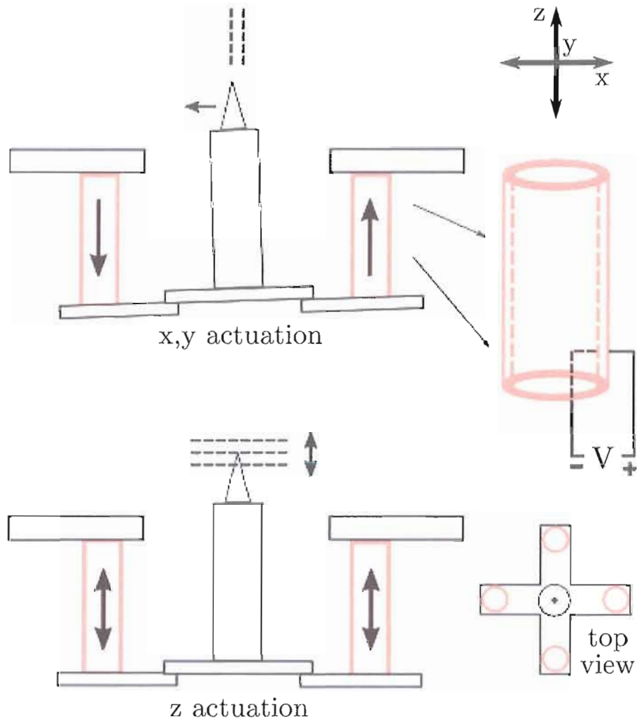
Figure 11: Actuating the probe tip. The tubes opposite one another work together to move the tip. As one tube expands, its counterpart contracts, causing the central post to rock in a plane. For small displacements this translates into lateral movement of the tip. Moving the tip towards (or away) from the surface requires an identical contraction (or extension) from all four of the piezoelectric tubes. The top view shows the four quadrant geometry of the rocker with the probe tip in the center and the piezoelectric tubes at the four quadrants. Also shown on the right is a schematic for applying the voltage. Electrodes are soldered to nickel plating on the inside and the outside of the piezoelectric tube walls. A tube contracts when a voltage is applied across the walls of the tube with the polarity shown above. In operation, the quiescent voltage across the tube walls is set to about 80 volts. Contraction and expansion of the tubes is obtained by increasing or lowering the voltage respectively.
