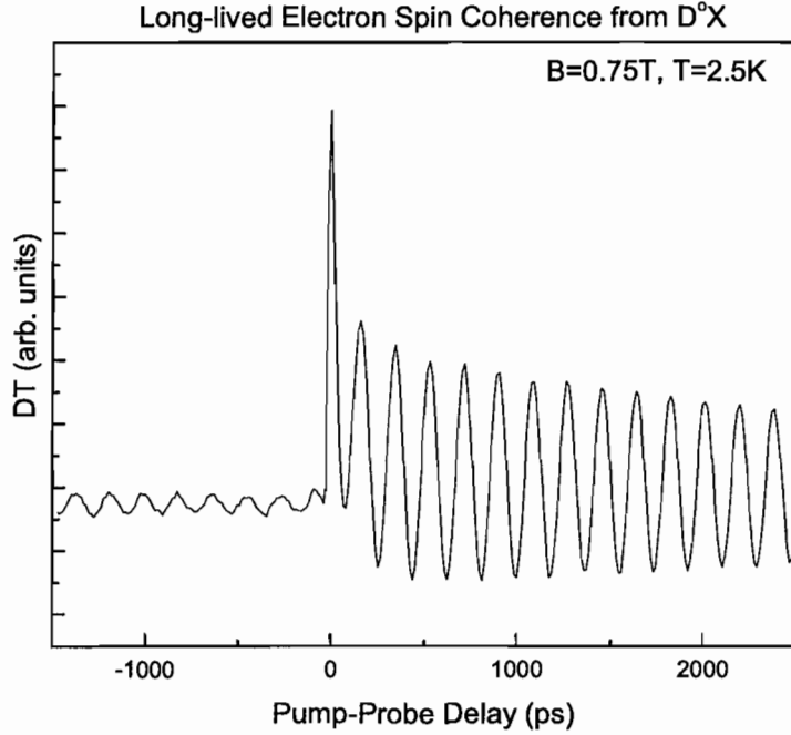
Figure 5.5: Long-lived QBs from Donor-Bound Electrons. Spin coherence from D^0 observed in the DT as long-lived quantum beats. The oscillatory signal present at negative delay times are quantum beats initialized in the previous pump cycle, 12 ns earlier.
