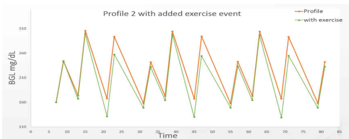
Figure 25 : Profile 2.2 BGL reading after adding Exercise
