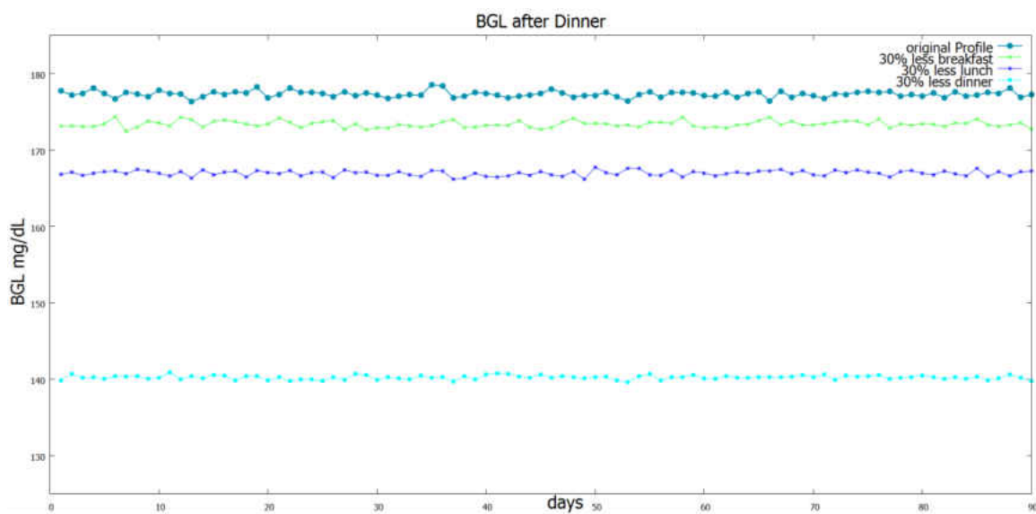
Figure 49 : profile-4 BGL after dinner with reduced diet
