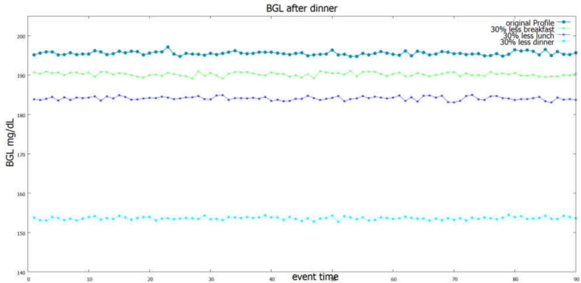
Figure 38 : Profile-3 BGL after dinner for 90 days with reduced diet
