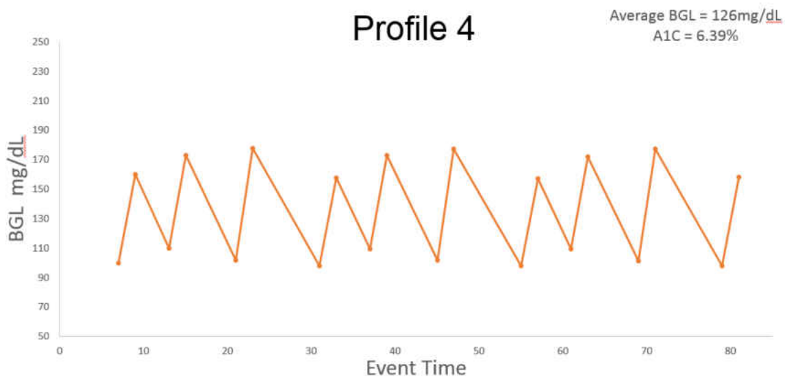
Figure 45 : profile-4 BGL reading before and after each events
