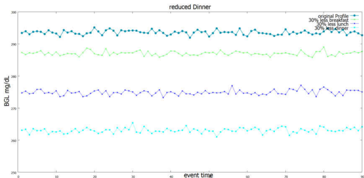
Figure 24 : Profile 2 BGL after dinner with reduced diet
