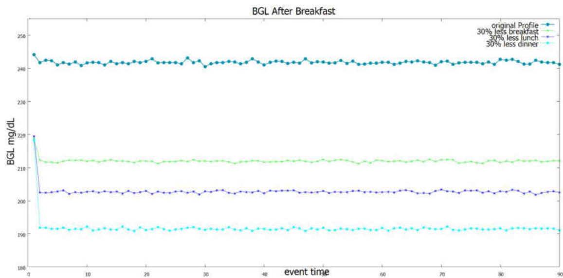
Figure 21 : Profile 2 BGL after breakfast with reduced diet
