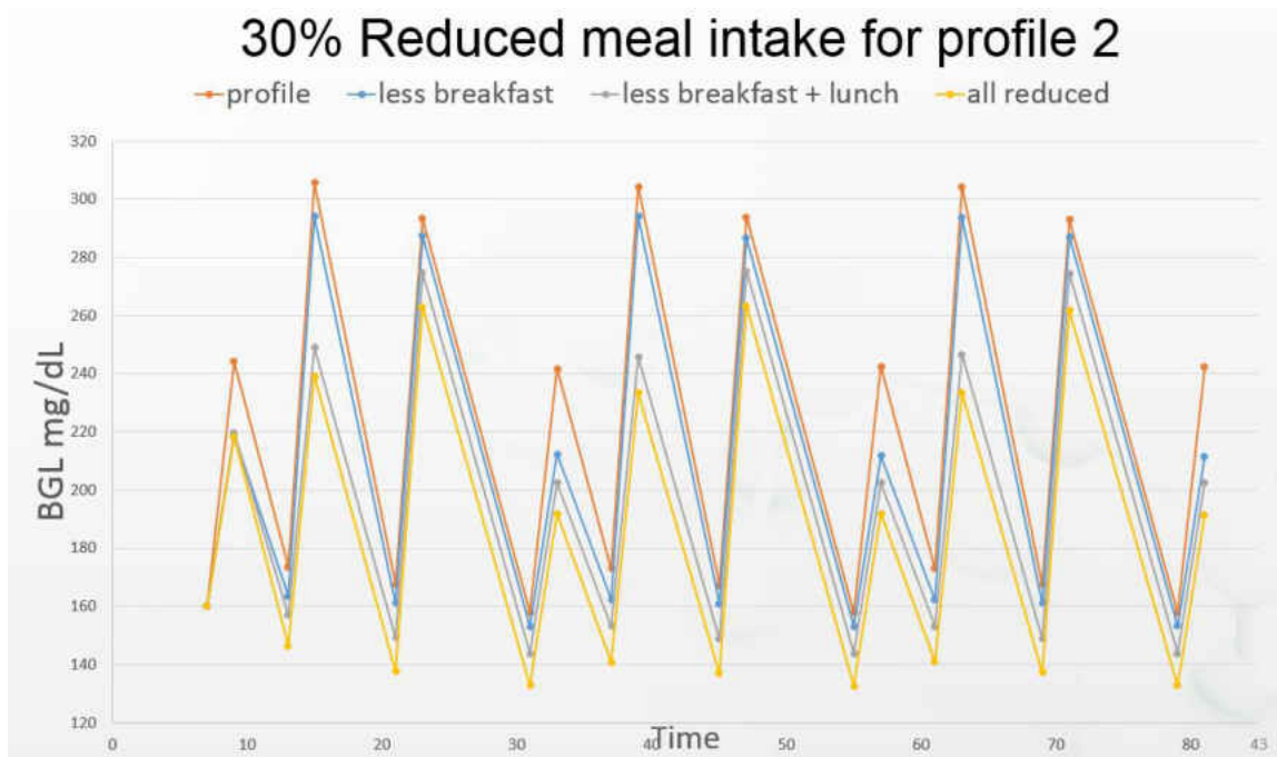
Figure 19: Profile 2 BGL after reduced meal intake
