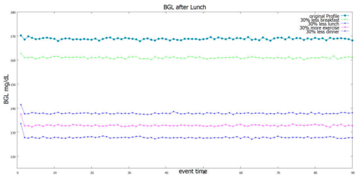
Figure 57 : Profile-4.2 BGL after lunch with reduced diet
