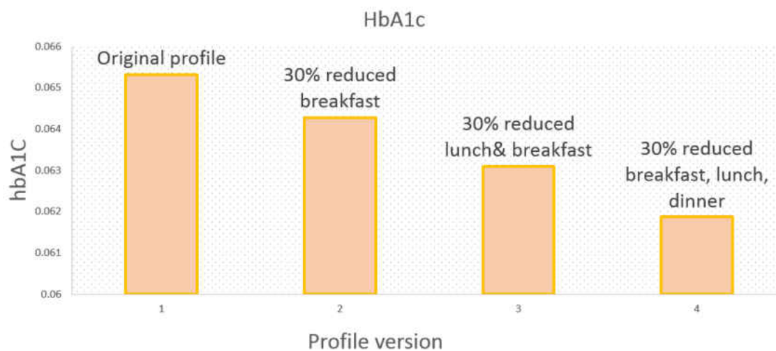
Figure 34 : Profile-3 HbA1C value with reduced meal intake
