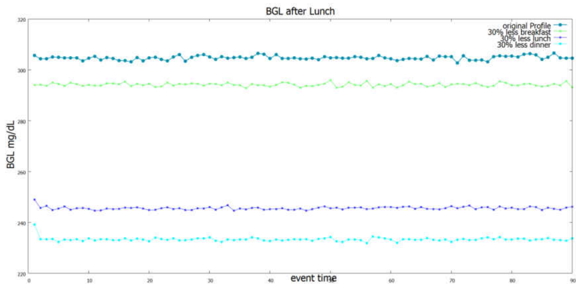
Figure 23 : Profile 2 BGL after lunch with reduced diet
