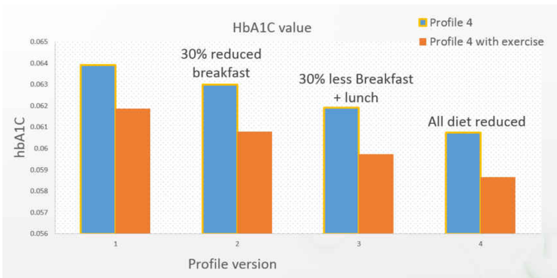
Figure 53 : Profile 4 vs Profile 4.2 HbA1C value
