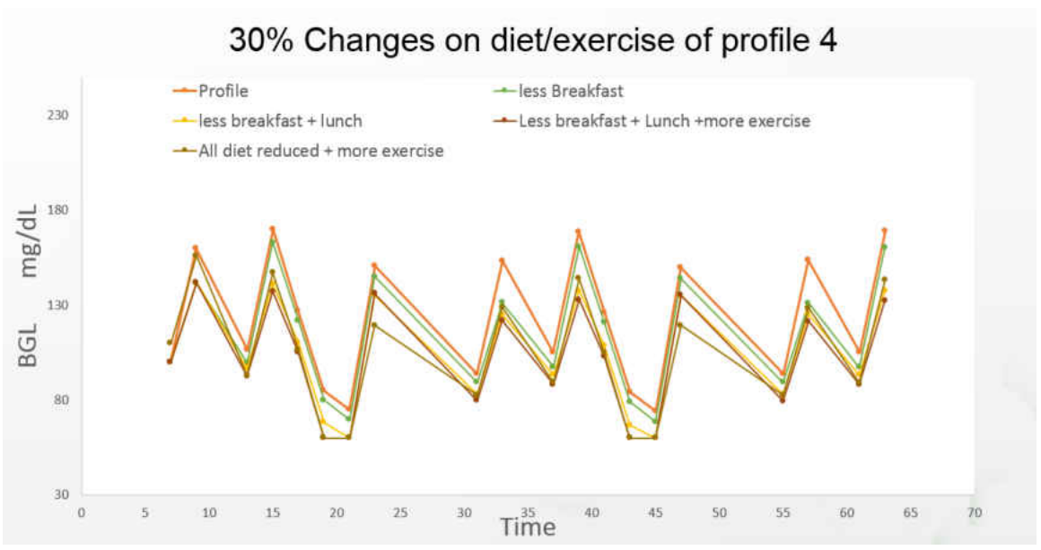
Figure 55 : Profile-4.2 BGL before and after each events with added exercise and with reduced diet
