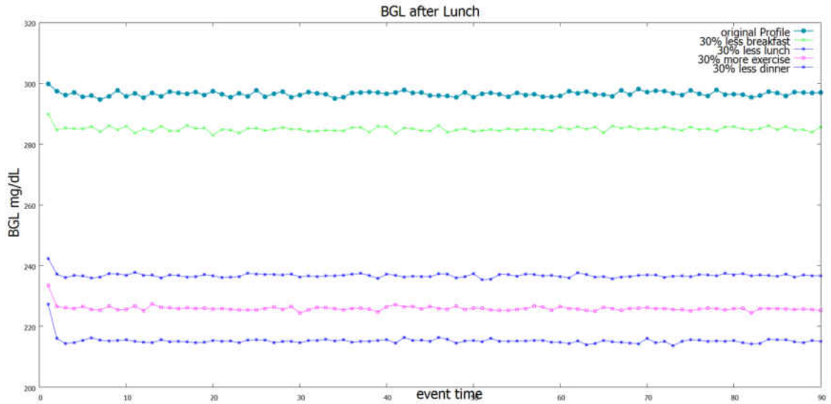
Figure 30 : Profile 2.2 BGL after lunch with reduced diet
