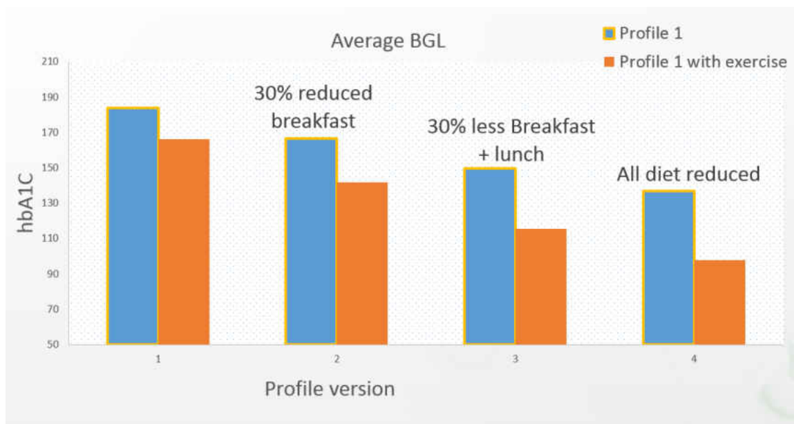
Figure 15 : Profile 1 average BGL vs. Profile 1.2 Average BGL
