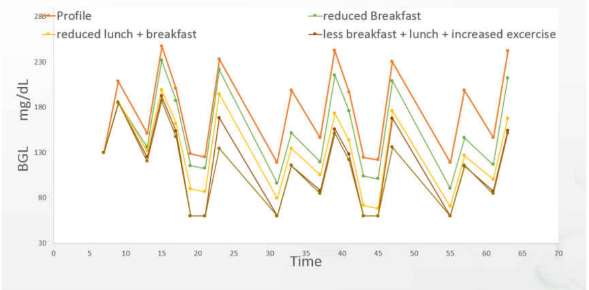
Figure 13 : Profile 1.2 reading of BGL before and after every events after adding exercise
