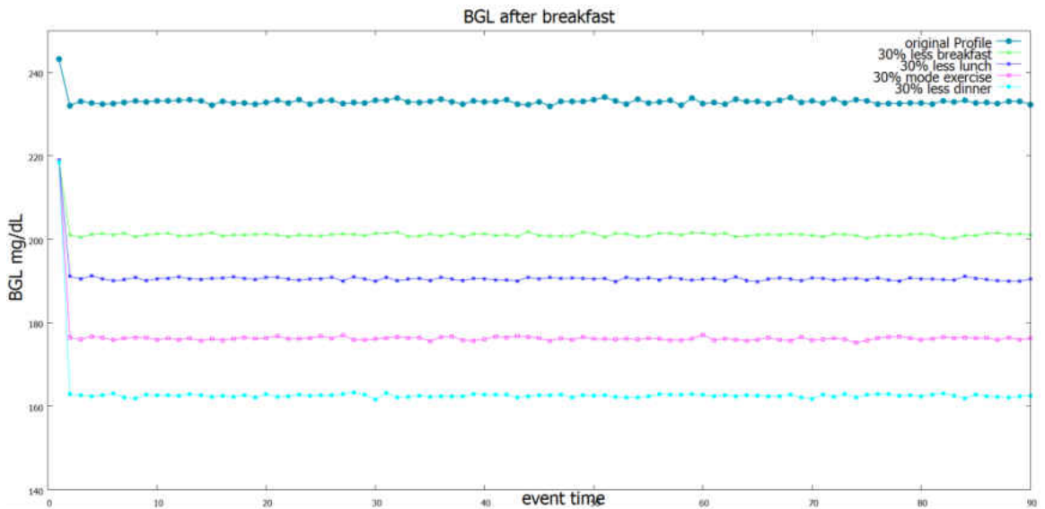
Figure 31 : Profile 2.2 BGL after breakfast for 90 days with reduced diet
