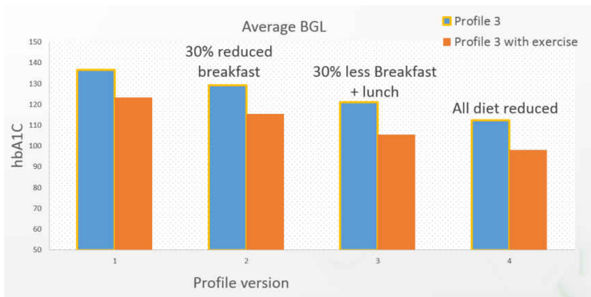
Figure 41 : Profile 3 vs. Profile 3.2 average BGL
