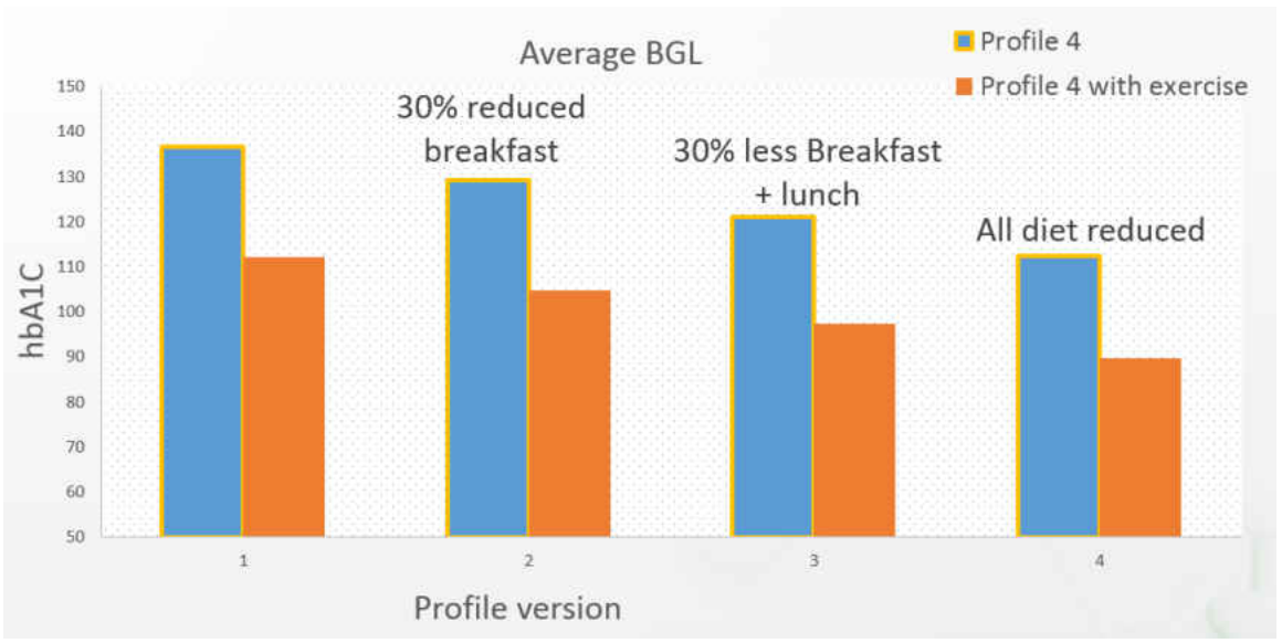
Figure 54 : Profile 4 vs Profile 4.2 average BGL
