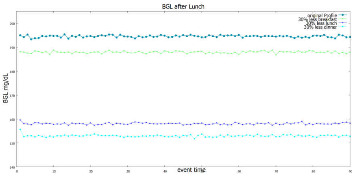
Figure 37 : Profile-3 BGL after lunch for 90 days with reduced diet
