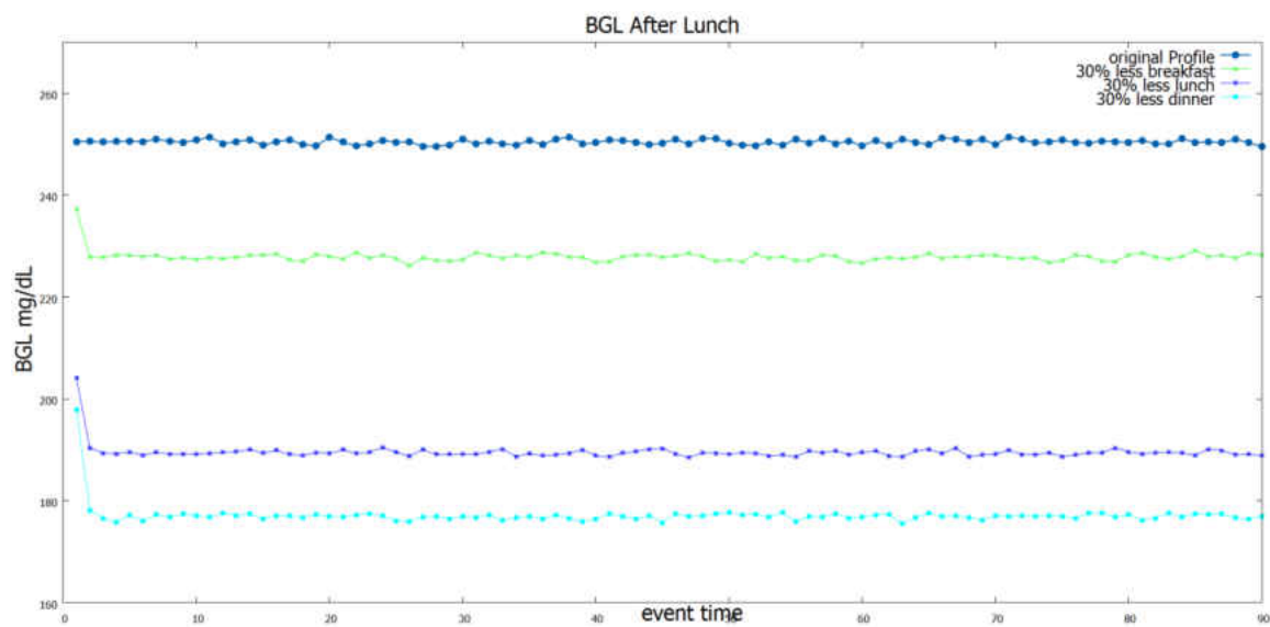
Figure 10 : Profile-1 BGL after lunch for reduced diet
