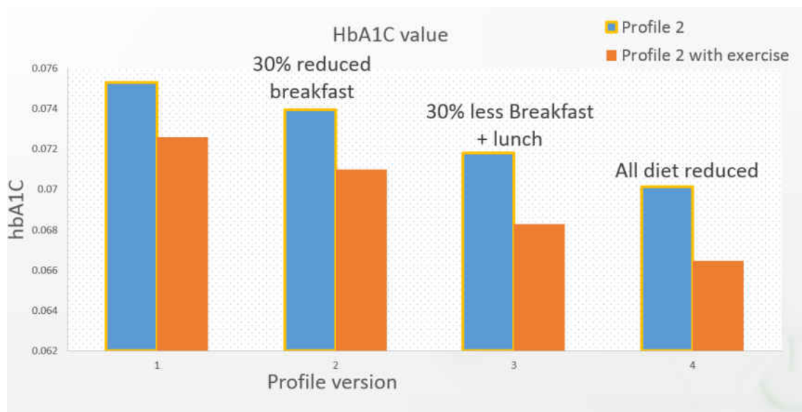
Figure 26 : Profile 2.2 A1C value with exercise event and reduced diet
