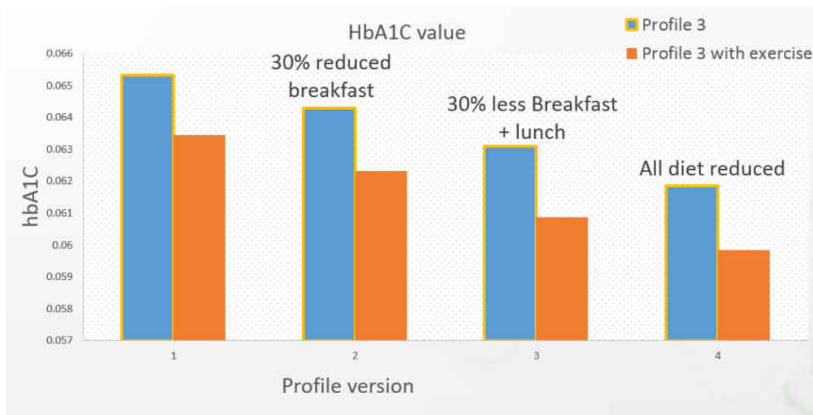
Figure 40 : Profile 3 HbA1C vs. Profile 3.2 HbA1C
