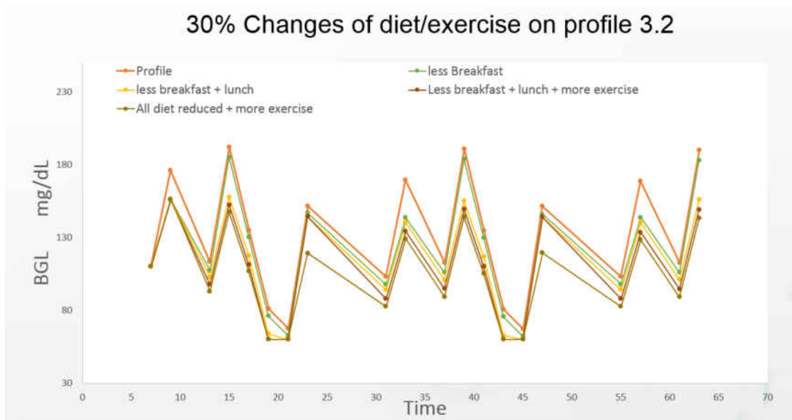
Figure 42 : Profile 3.2 BGL before and after every event with reduced meal and increased exercise
