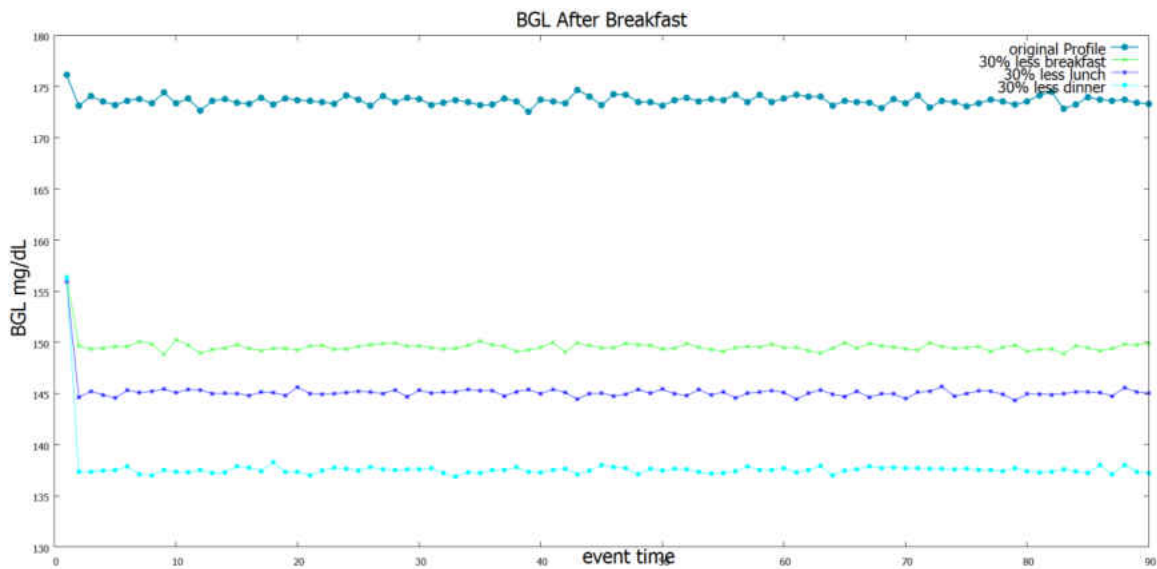
Figure 36 : Profile-3 BGL after breakfast for 90 days with reduced diet
