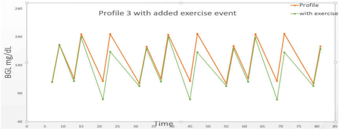
Figure 39 : profile 3.2 generated from profile 3 after adding exercise event
