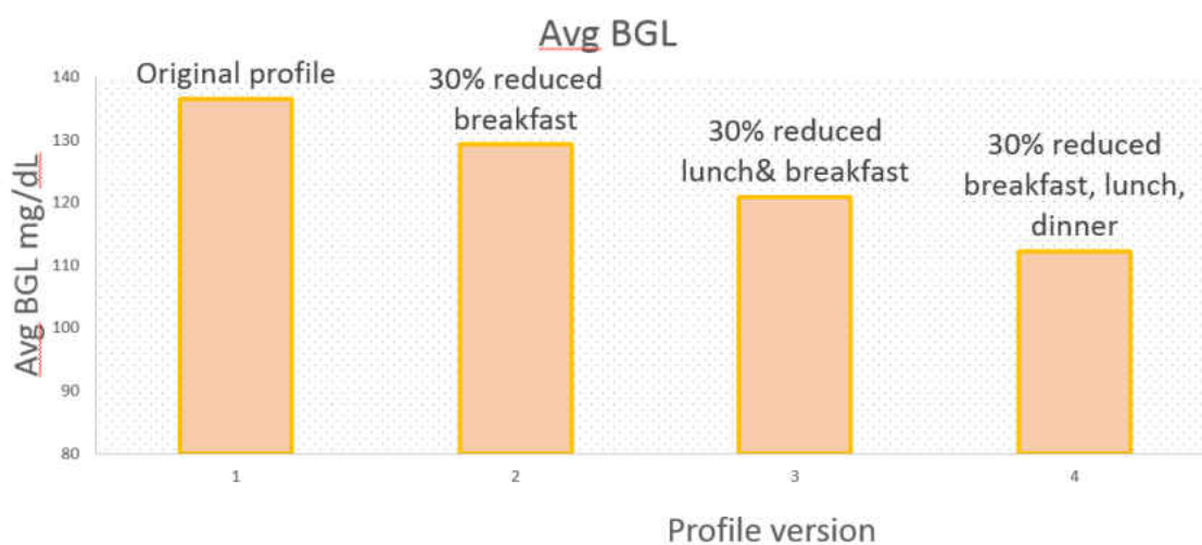
Figure 35 : Profile-3 average BGL with reduced meal intake
