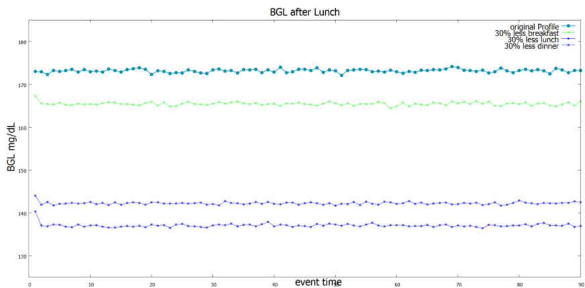
Figure 51 : profile-4 BGL after lunch with reduced diet
