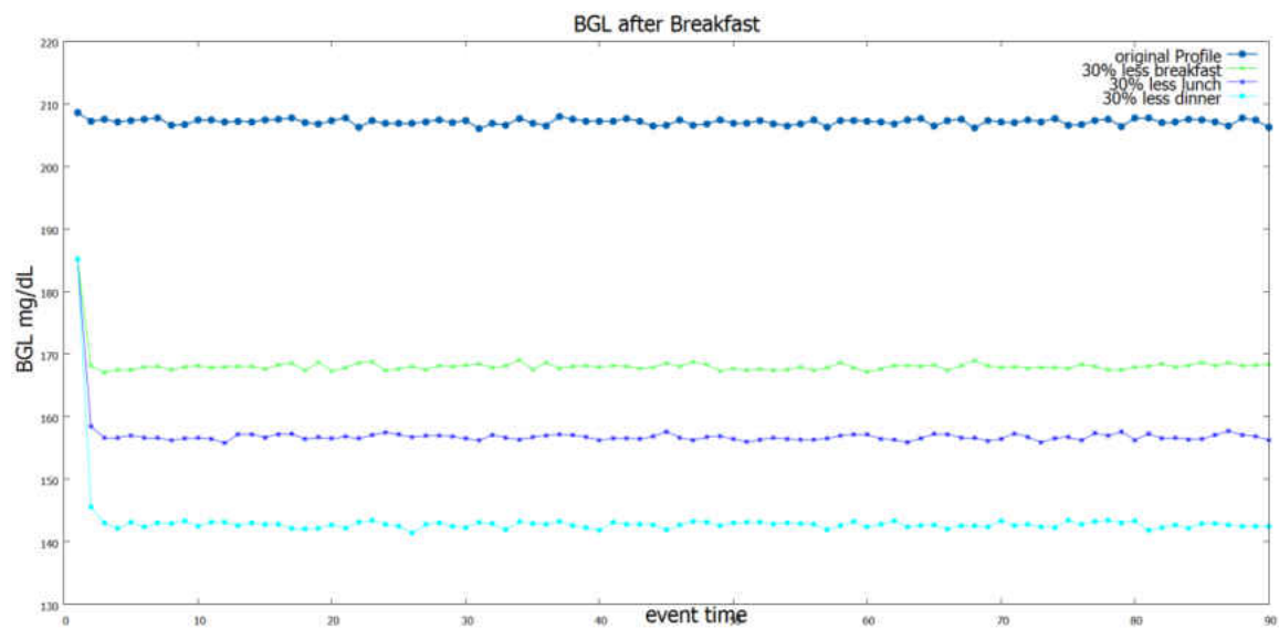
Figure 9 : Profile-1 BGL after breakfast for reduced food
