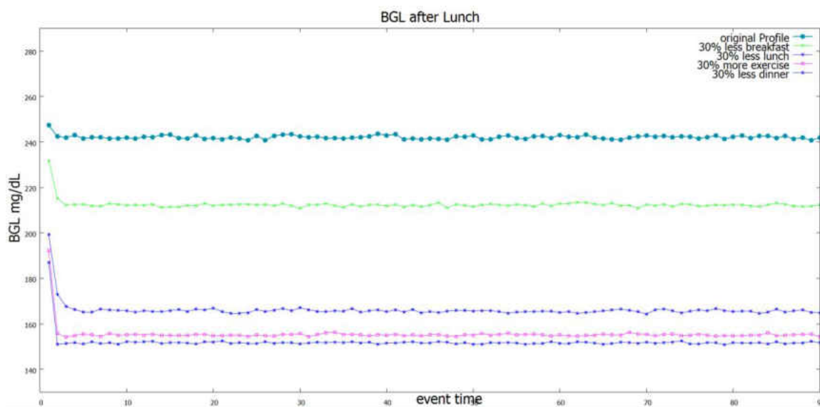
Figure 16 : Profile 1.2 BGL after Lunch
