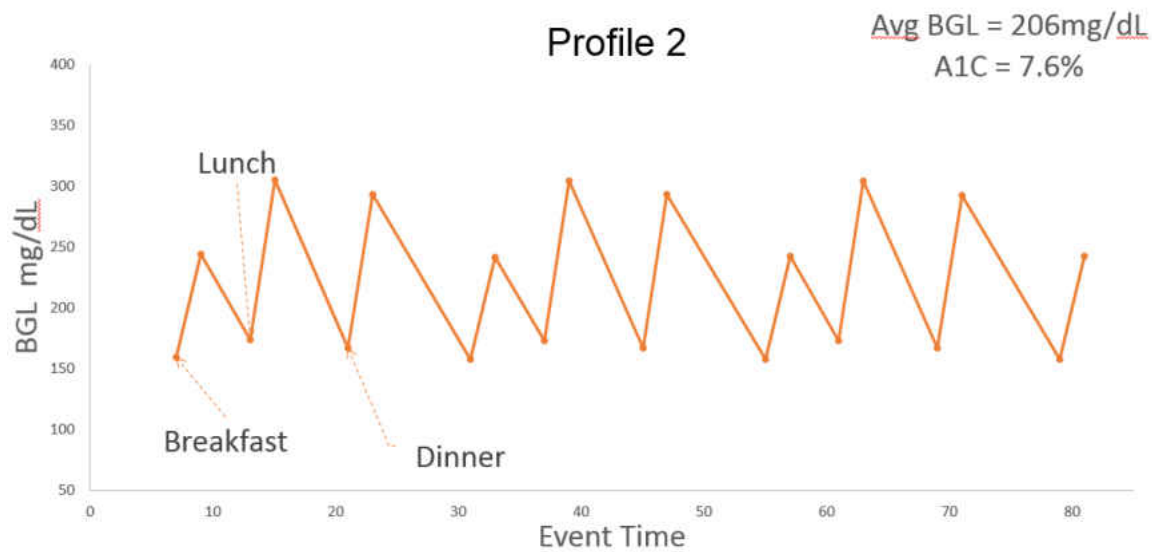
Figure 18 : BGL after different events for profile 2
