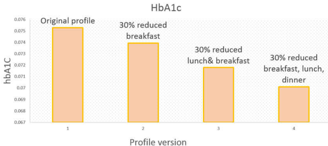
Figure 20 : Profile 2 HbA1C value after modification of meal intake
