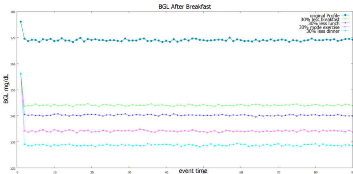
Figure 43 : Profile 3.2 BGL after breakfast with reduced diet for 60 days
