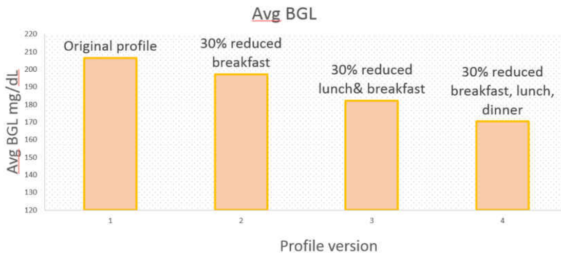
Figure 22 : Profile 2 average BGL changes with diet change
