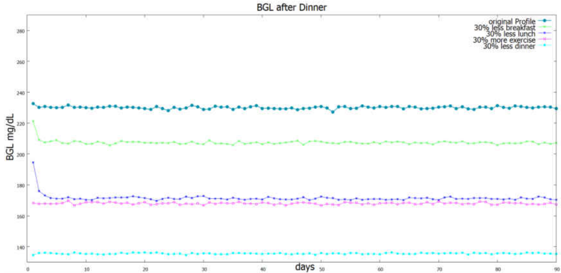
Figure 17 : Profile 1.2 BGL after dinner
