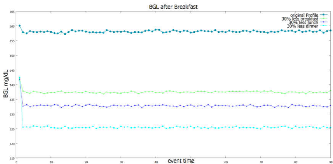
Figure 50 : profile-4 BGL after breakfast with reduced diet
