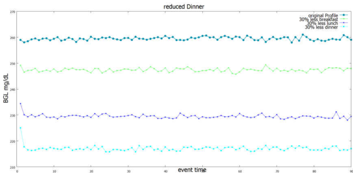
Figure 11 : Profile-1 BGL after dinner for reduced diet
