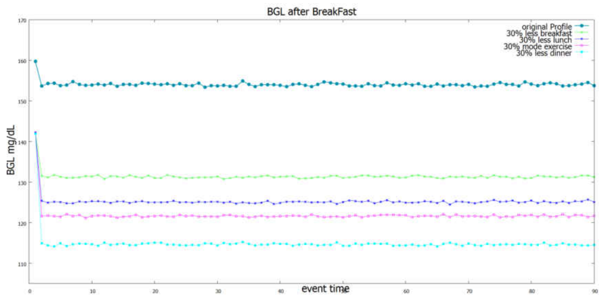
Figure 56 : Profile-4.2 BGL after breakfast with reduced diet
