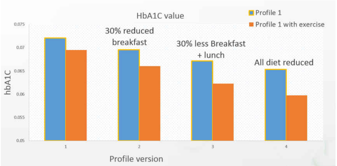
Figure 14 : Profile 1 HbA1C vs. Profile 1.2 HbA1C
