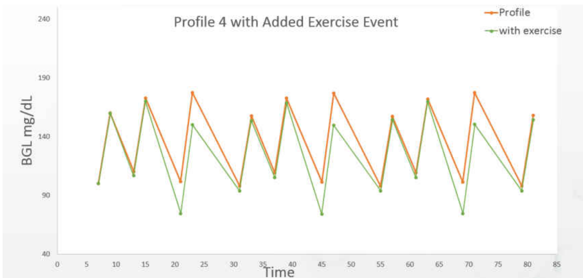
Figure 52 : profile 4.2 generated from profile 4 after adding exercise event
