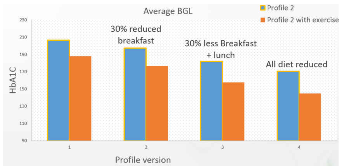
Figure 26 : Profile 2.2 A1C value with exercise event and reduced diet
