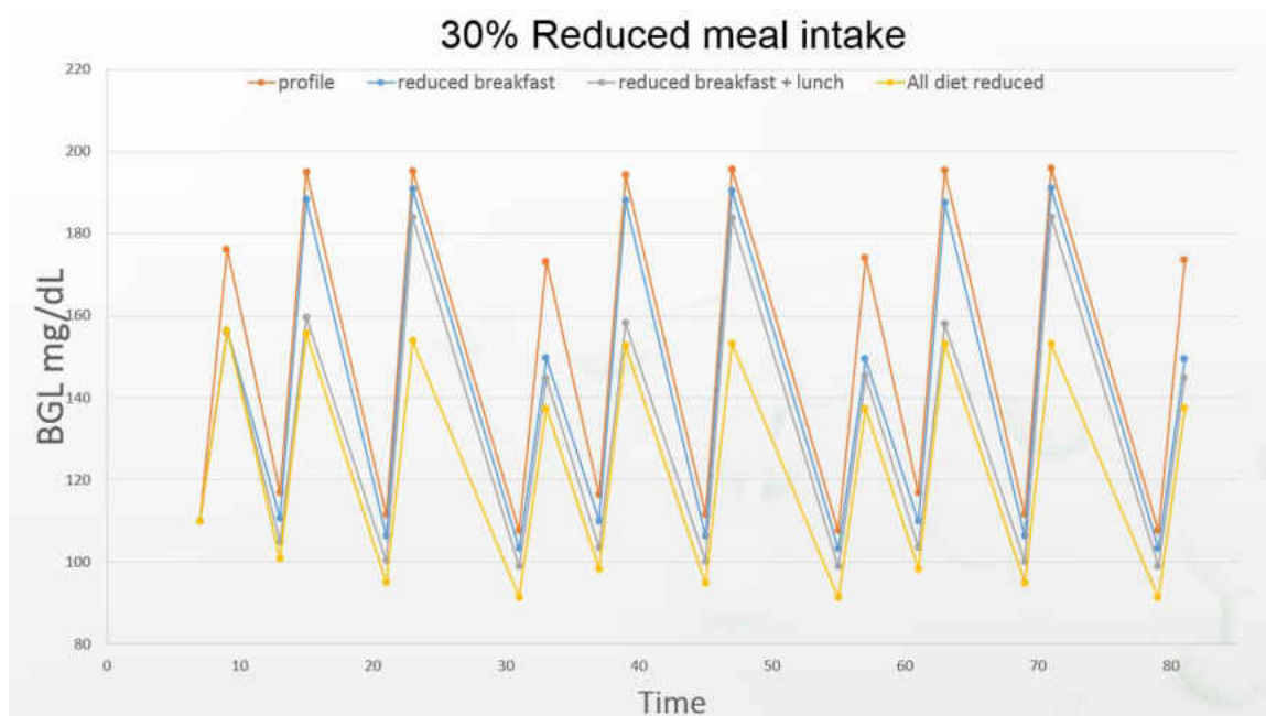
Figure 33 : Profile-3 BGL level after every event with reduced diet for profile 3
