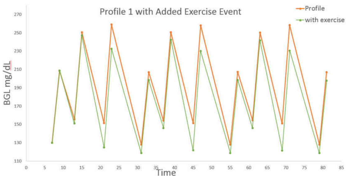
Figure 12 : Profile 1.2 BGL after adding exercise before dinner
