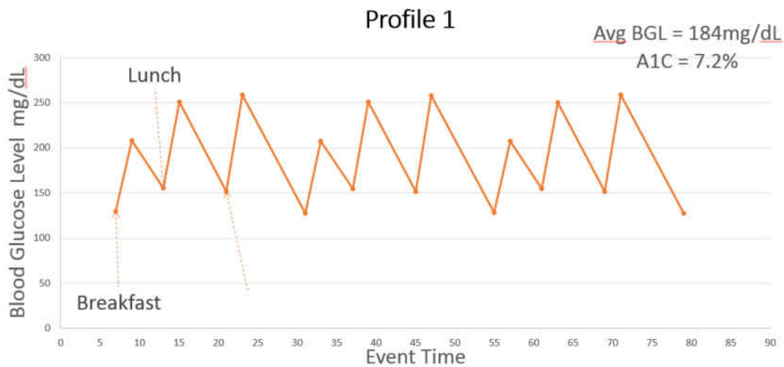
Figure 5 : Profile 1 blood glucose level after different events
