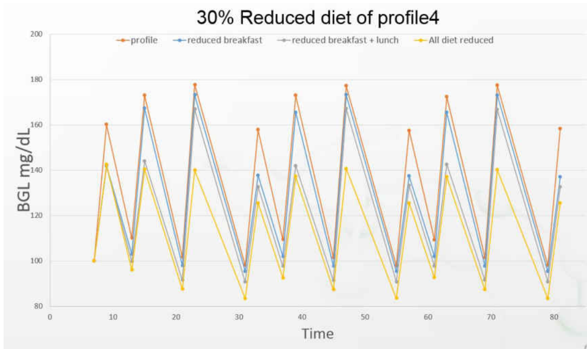
Figure 46 : profile-4 BGL reading before and after each event with reduced meal
