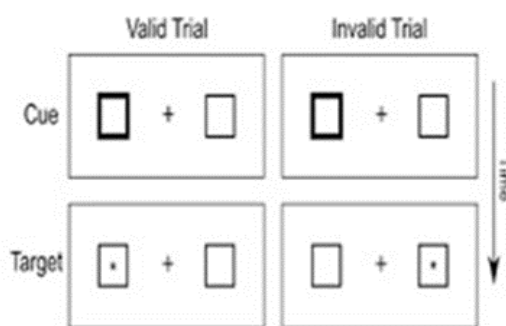
Figure 1. Posner-cueing task.
