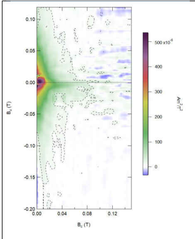
C-15 - 300°C 15 days; Rhyolitic Glass
