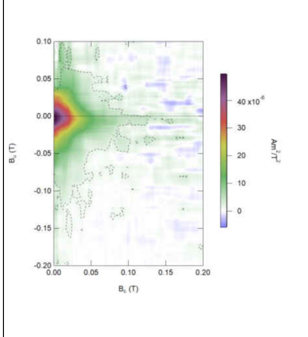
C-25 - 450°C 1 day; Rhyolitic Glass
