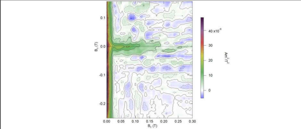
Basalt 400°C
