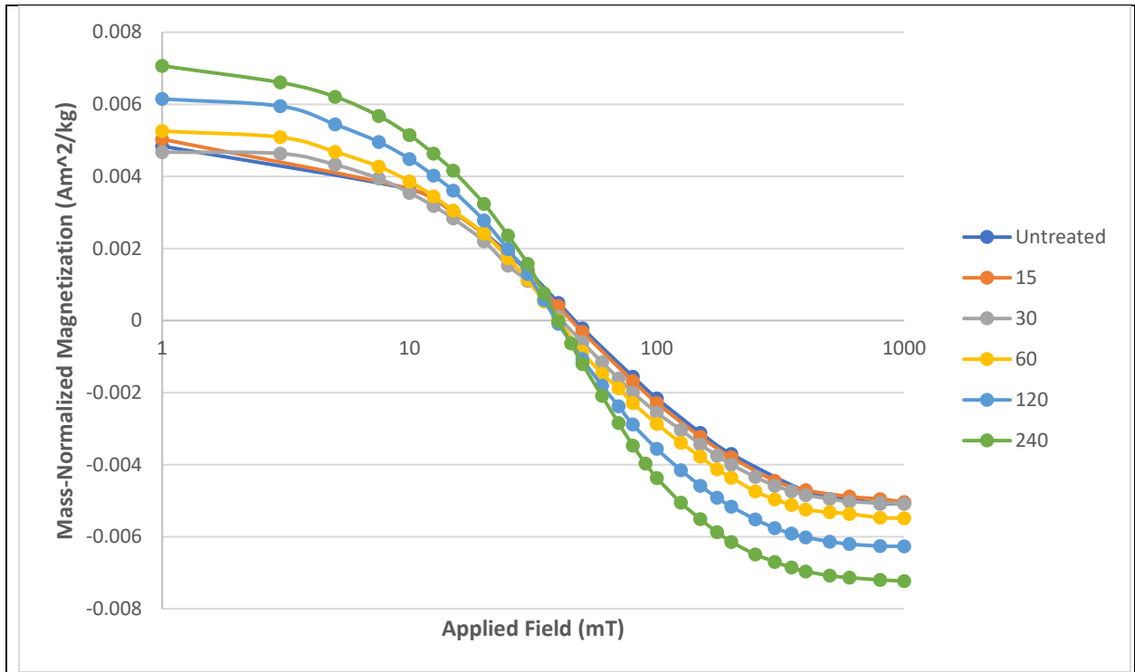
Basalt – 300°C
