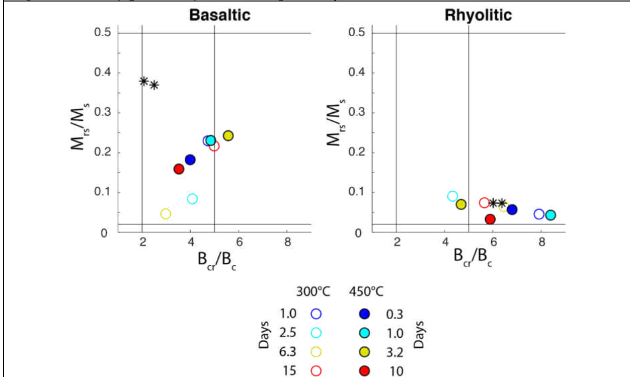
Figure 3.19: Day plots of hydrated samples (Day et al., 1977)
