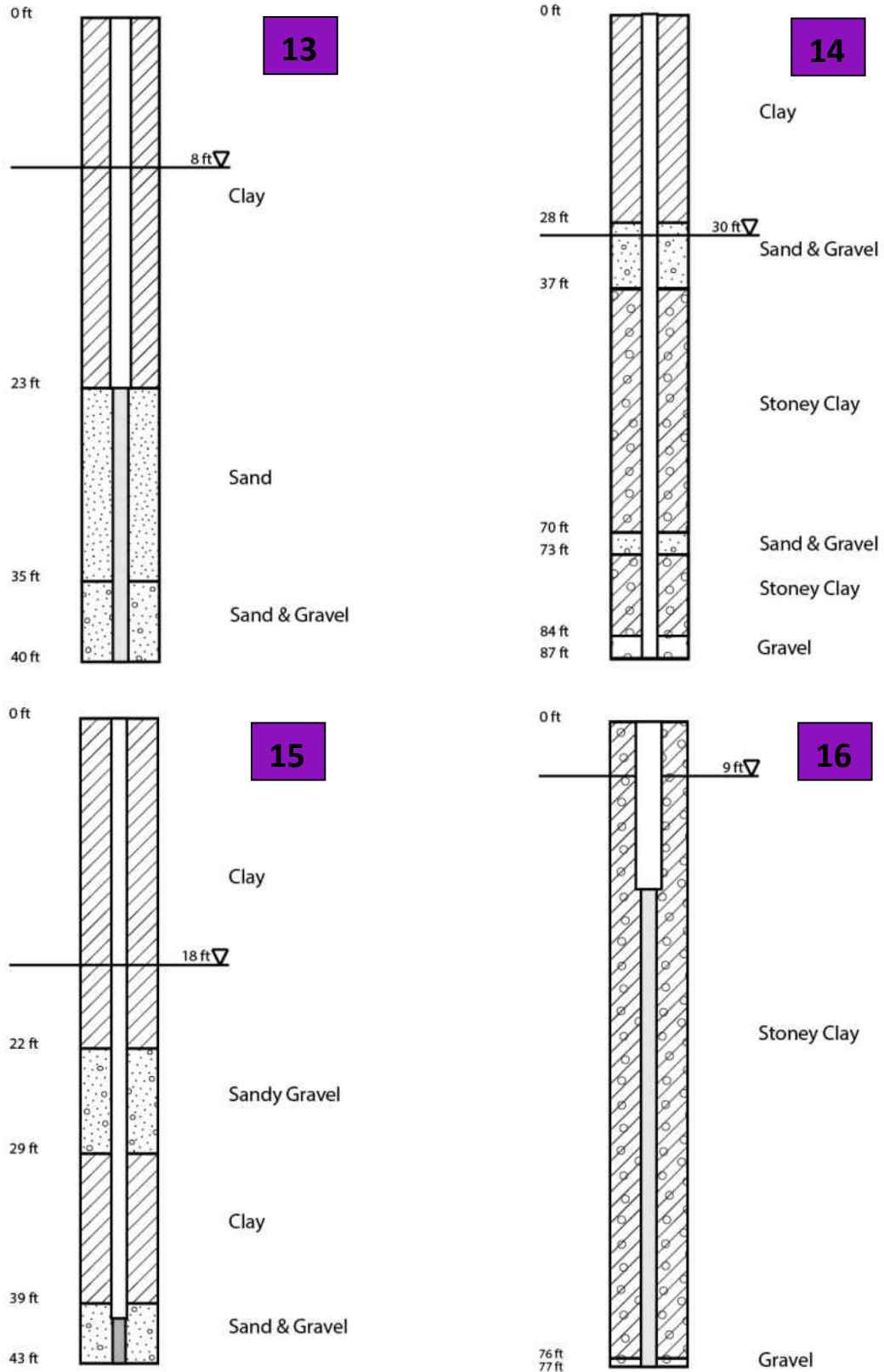
Figure 9d: Well Logs for Waukesha County. Well ID 13, 14, 15, 16 Depicted in Purple in Figure 7.
