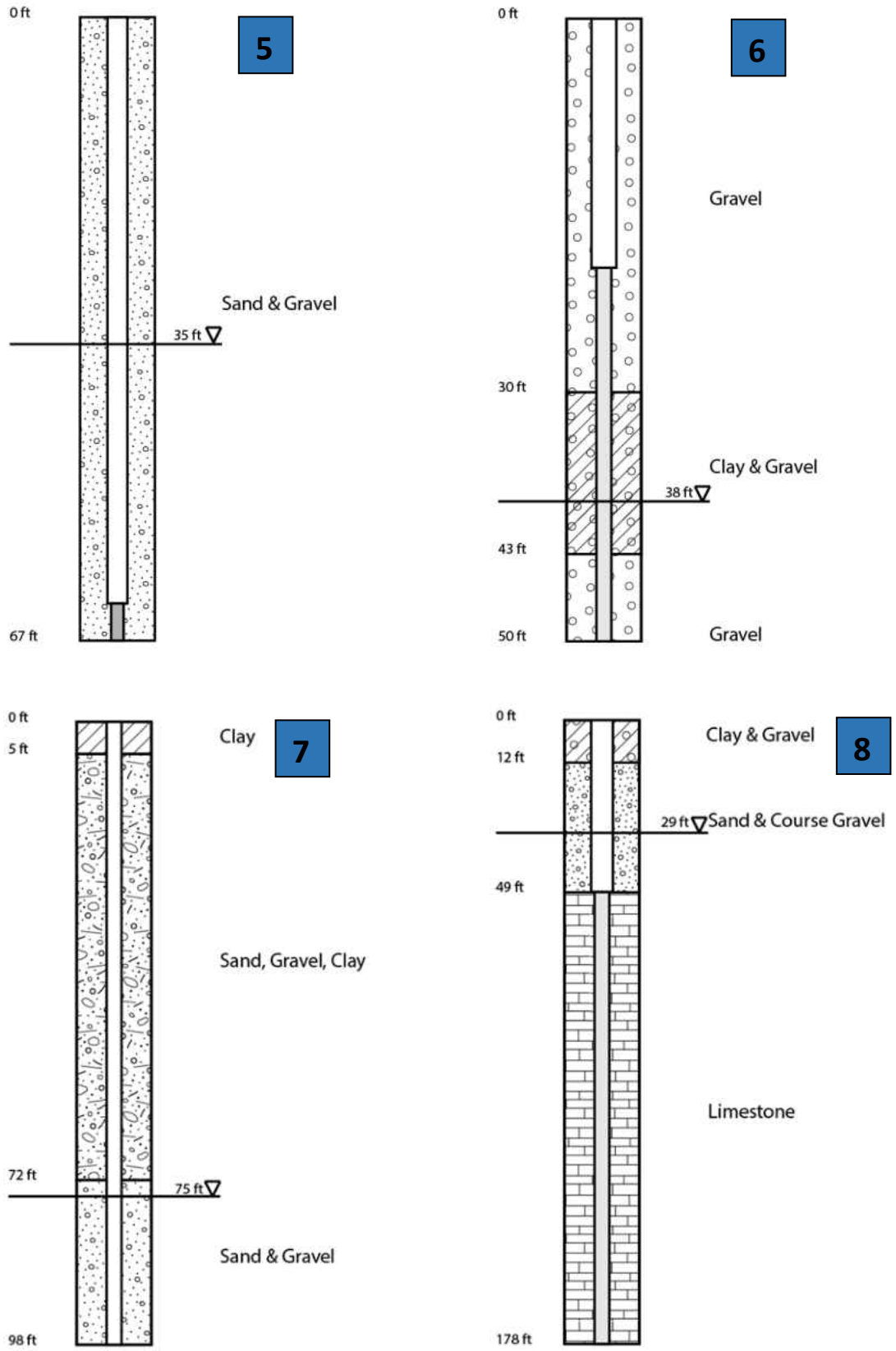
Figure 9b-1: Well Logs for Washington County. Well ID 5, 6, 7, 8. Depicted in Blue in Figure 7.
