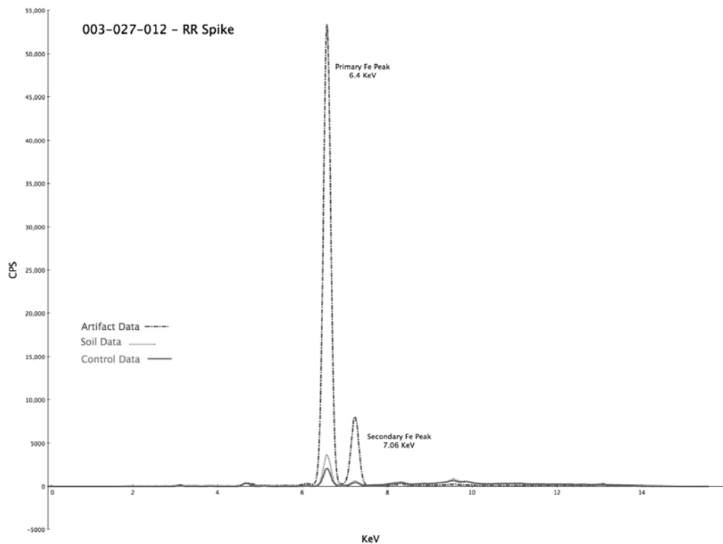
Figure 22. Example of an XRF spectral curve.
