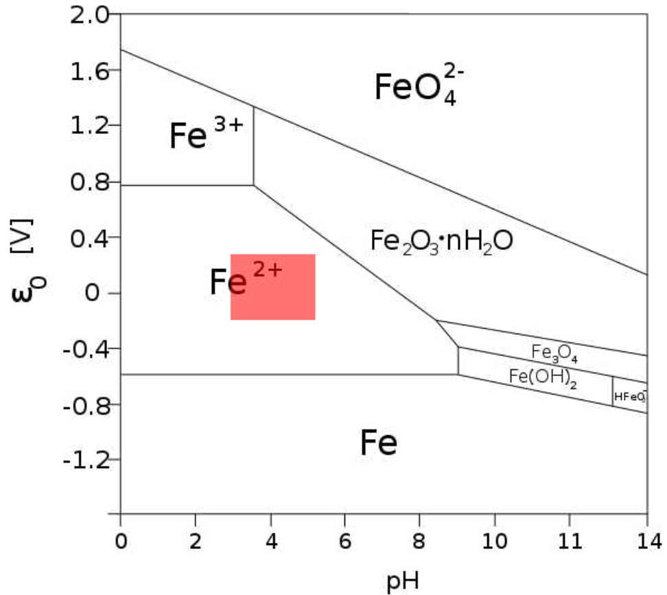
Figure 28. The shaded area on the diagram represents the soil conditions found at Camp Lawton.
