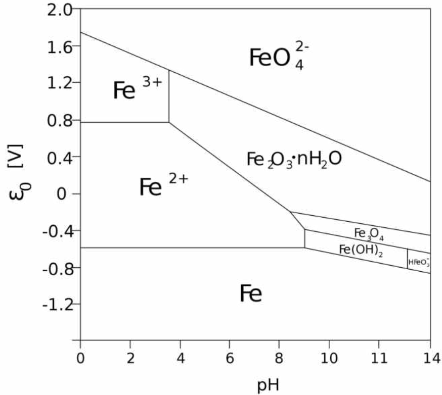
Figure 1. This is a Pourbaix diagram showing the relationship between pH and reduction potential and the ensuing iron reactions that occur.
