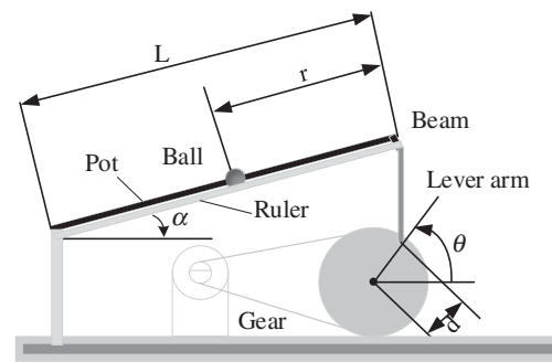
Figure 1. Mechanical structure of the ball and beam system.
