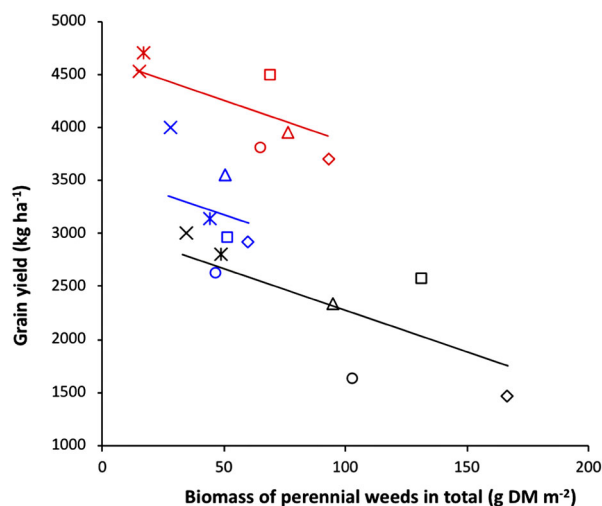
Figure 1. The relationships between biomass of perennial weeds in total (g DM m -2 ) and grain yield (kg ha -1 ) of spring barley in 2014 (blue colour), spring oat in 2015 (red) and spring wheat in 2016 (black) in experiment I. The relationships can be described by one common slope -7.82 (kg ha -1 g -1 m 2 ) and three intercepts: 2014 = 3569.3 (kg ha -1 ), 2015 = 4643.2 (kg ha -1 ), 2016 = 3060.0 (kg ha -1 ). Non-transformed weed biomass values was used in the regression. \diamond = 1 , \circ = 2 , \square = 3 , \times = 4 , \Delta = 5 and \times = 6 .
