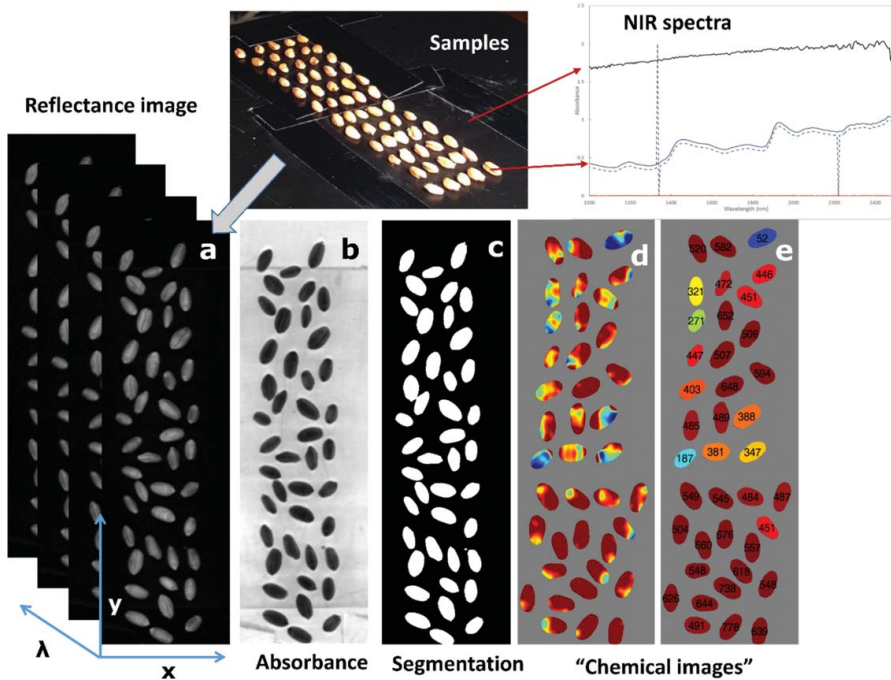
Figure 2. Example of hyperspectral images (‘‘hypercubes’’) obtained by HSI, showing wheat kernels. The samples are presented on the acquisition stage, with indication of the reflectance spectrum at one pixel belonging to the black plastic stage (background), and one pixel belonging to a wheat kernel. The dotted line indicates the spectrum before the spike correction. (a) Reflectance image at a particular wavelength, showing the three-dimensional structure of the hypercube. (b) Absorbance image, for the same image, and (c) segmentation necessary to remove the background and select the region of interest for further analyses. (d) Application of a quantitative prediction at a single pixel level, obtaining the so-called ‘‘chemical image’’ (colors indicate different concentrations of a compound); (e) calculation of the average content of a compound or property on a single kernel level (numbers indicate the predicted Hagberg Falling Number, as in Caporaso et al. (44)).
