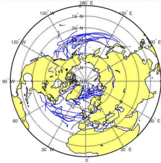
Storm Tracks for top 50 Vorticity-centered Storms in the Early 2010s
