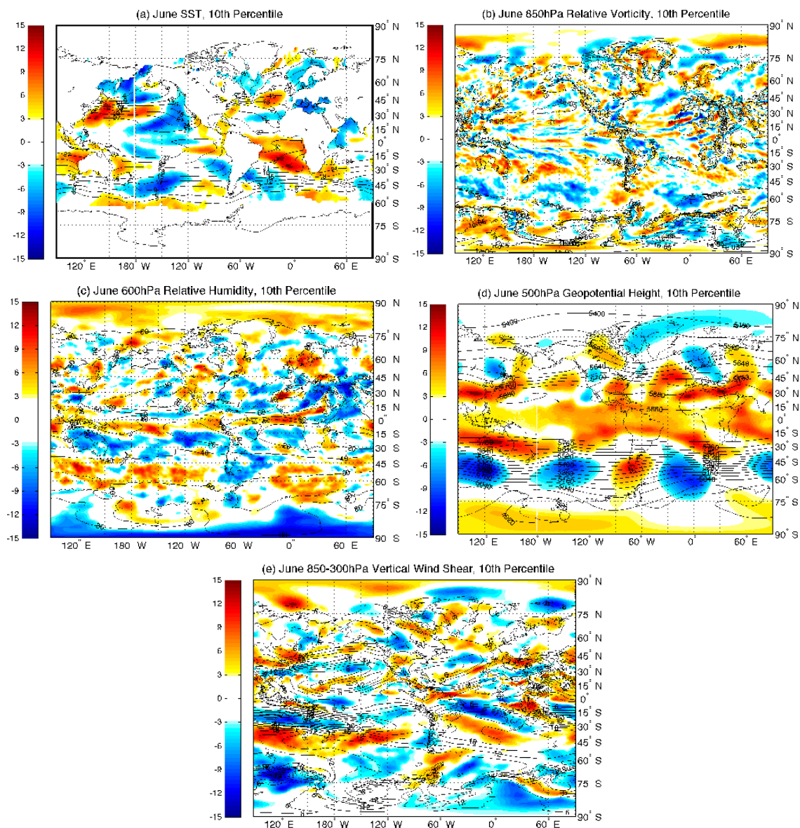
Figure 4. Linear regression (colored shading) of the 10 th percentile formation date for each Atlantic TC season against June monthly-mean (a) SST ( ^{\circ}\text{C} ), (b) 850hPa relative vorticity ( \times 10^{-5} \text{ s}^{-1} ), (c) 600hPa relative humidity (%), (d) 500hPa geopotential height (m), and (e) 850-300hPa vertical wind shear magnitude ( \text{m s}^{-1} ). Blue shading indicates a shift towards an earlier start date while red shading indicates a shift towards a later start date with a one standard deviation increase in the stated variable. Relative vorticity values are opposite in the southern hemisphere. Contours show composite (1979-2013) June monthly-mean values for each variable.
