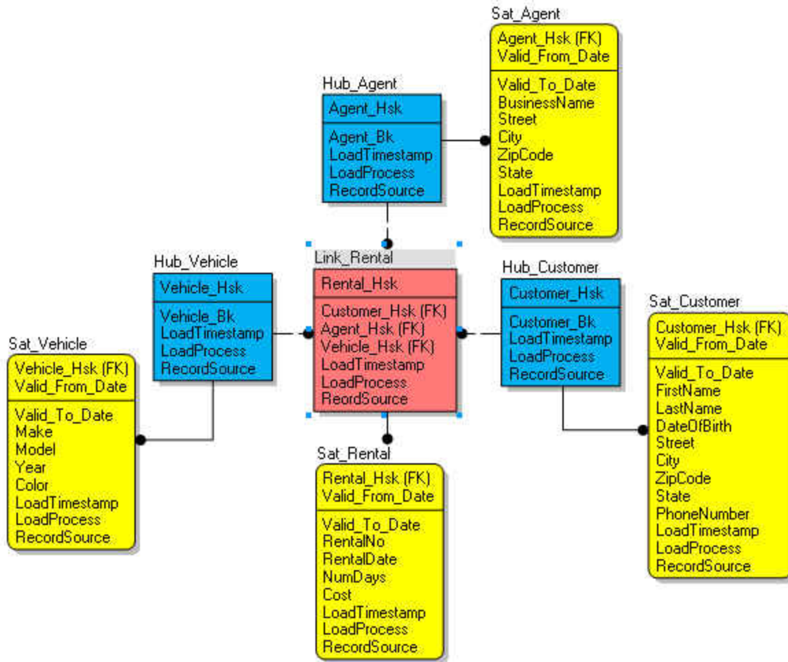
Figure 7-7 Data Vault (2.0) model for the Rental Company (simplified)
