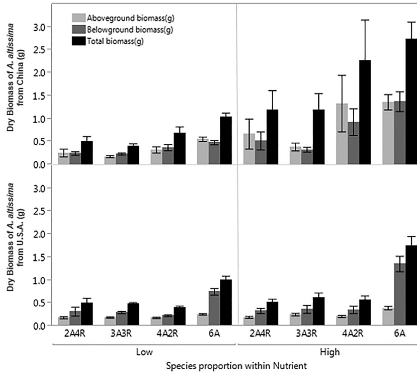
Figure 1. Aboveground, belowground and total biomass of Ailanthus altissima in a full-factorial substitutive design experiment with Robinia pseudoacacia at constant density (six plants per 8 L pot). The solid bars and error bars represent the average biomass per A. altissima plant and the standard error within each treatment group. The upper graph represents the results from an experiment using A. altissima seedlings from a Chinese seed lot, and the lower graph represents A. altissima seedlings grown from a West Virginia, US seed lot. Two nutrient levels (low and high) were used for the experiment, along with the four different proportions of A. altissima and R. pseudoacacia . (e.g. 2A4R=two A. altissima and four R. pseudoacacia seedlings; 3A3R=three A. altissima and three R. pseudoacacia seedlings).
