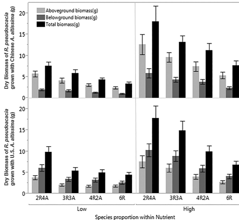
Figure 2. Aboveground, belowground and total biomass of Robinia pseudoacacia seedlings in a full-factorial substitutive design experiment with Ailanthus altissima at a constant density (six plants per 8 L pot). The solid bars and error bars represent the average biomass per R. pseudoacacia plant and the standard error within each treatment group. The upper graph represents the results from an experiment using A. altissima seedlings from a Chinese seed lot, and the lower graph represents using A. altissima seedlings grown from a West Virginia, US seed lot. Two nutrient levels were used for the experiment, along with four different proportions of R. pseudoacacia and A. altissima seedlings. (e.g. 2R4A = two R. pseudoacacia and four A. altissima seedlings; 3R3A = three R. pseudoacacia and three A. altissima seedlings).
