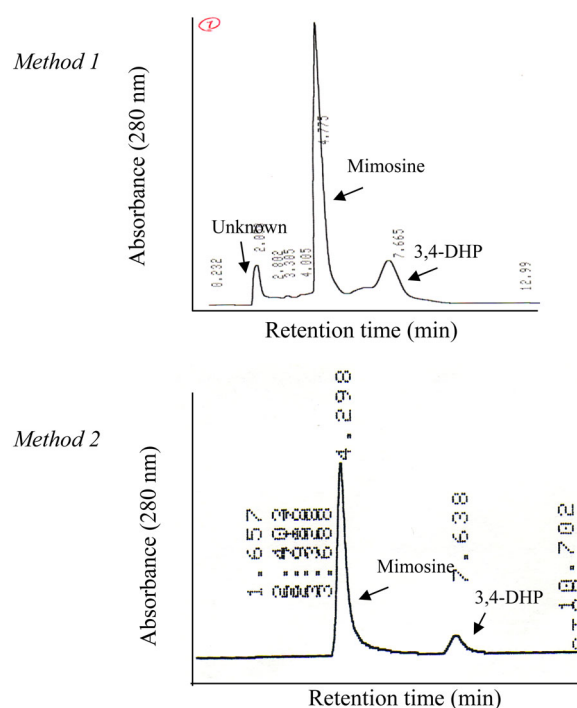
Figure 2. Mimosine and its degraded product 3,4-DHP in the HPLC profile. Method 1: From young Leucaena leaves; Method 2: By oil bath. HPLC (Shimadzu) solvents: 10 mM KH 2 PO 4 ; 10 mM H 3 PO 4 ; acetonitrile = 45 : 45:10 (v/v), 0.1% sodium 1-octanesulfonate; Column: Jasco, C18 150 × 4.60 mm; Flow rate: 1 ml min -1 ; and Wave length: 280 nm.
