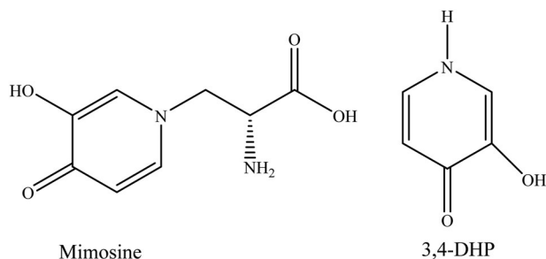
Figure 1. Chemical structures of mimosine and 3,4-DHP.
