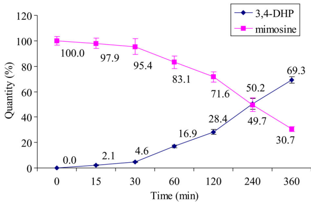
Figure 3. Correlative percentage of mimosine degraded to 3,4-DHP by high temperature. Bar values are mean ± SE (standard errors).
