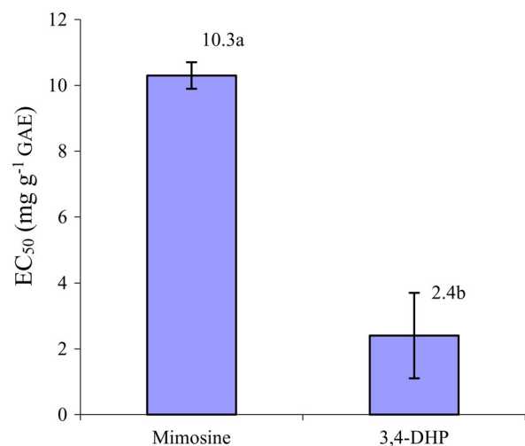
Figure 6. DPPH scavenging activity of mimosine and 3,4-DHP. Different letters in bars indicate significantly different ( P < .05 ) using Tukey's procedure. Bar values are the effective concentration ( EC_{50} ) of GAE ± SE.
