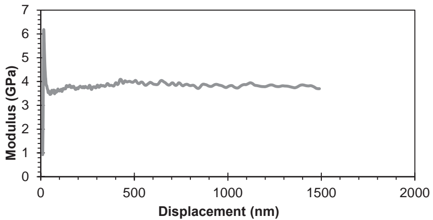
Figure B-29: Modulus vs. Displacement curve for 3 wt% xGnP ® -M-5 in Epoxy Test 32
