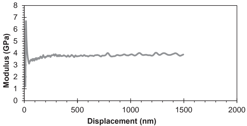
Figure B-26: Modulus vs. Displacement curve for 2 wt% xGnP ® -M-5 in Epoxy Test 26
