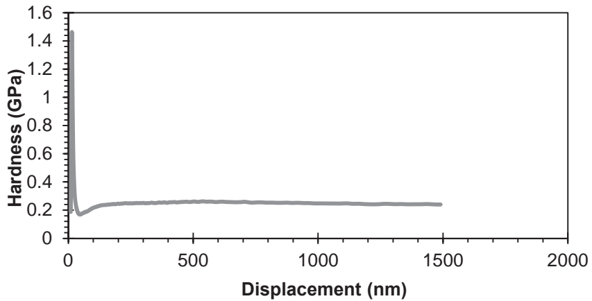
Figure B-15: Hardness vs. Displacement curve 4 wt% xGnP ® -M-15 in Epoxy Test 29
