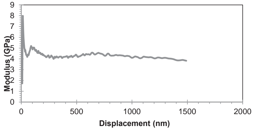
Figure B-17: Modulus vs. Displacement curve for 5 wt% xGnP ® -M-15 in Epoxy Test 13
