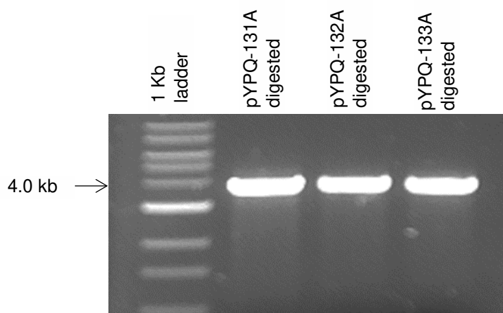
Figure 32: Second Digestion of Golden Gate Entry Plasmid DNA by BsmBI. DNA ladder (1kb) was used to estimate a product size 3808 bp.
