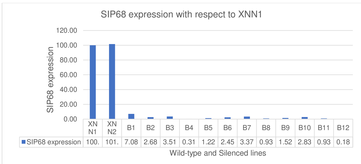
Figure 28: Densitometric Analysis of SIP68 Expression of T2 #B Line With Respect to XNN1. Signal is normalized to Ef1α intensity in each lane.
