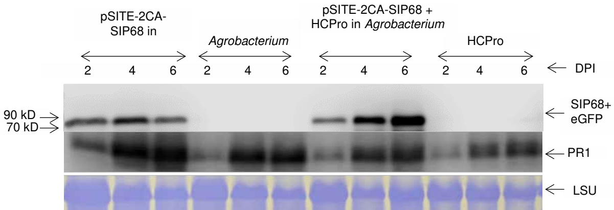
Figure 20: PR1 Protein Expressed by Agrobacterium, HCPPro and Agrobacterium+pSITE-2CA-SIP68 With and Without HCPPro at Different Time Points. Western blot analysis showing upper SIP68+eGFP protein expression (~82.53 kD), middle blot representing PR1 protein expression and the third representing corresponding coomassie blue stained blot showing large subunit of RuBisCo.
