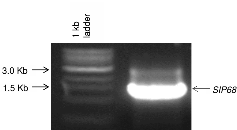
Figure 13: RT-PCR Amplification of SIP68 cDNA. Ethidium bromide stained 0.8% agarose gel showing ~1500bp amplified SIP68 cDNA. DNA ladder (1 kb) was used to compare the product size.
