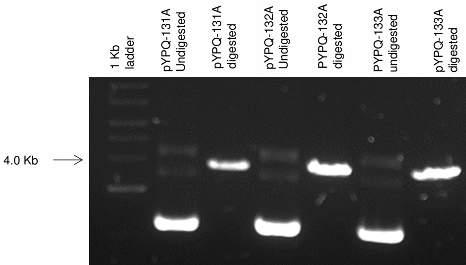
Figure 31: Golden Gate Entry Vector pYPQ131A, 132A, and 133A Digested by BgIII and Sall. DNA ladder (1 kb) ladder was used to compare product size (3808 bp).
