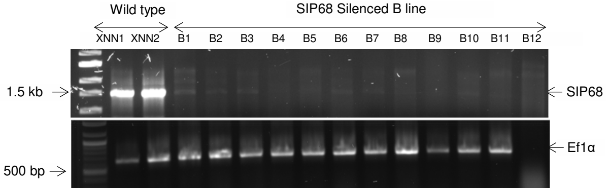
Figure 27: Screening of T2 RNAi Silenced #B Lines. Ethidium bromide stained 0.8% and 1% agarose gel showing expression of SIP68 and Ef1α respectively. DNA ladder (1 kb) for SIP68 (~1491bp) and 100 bp ladder for Ef1α (~600) was used to compare a product size.
