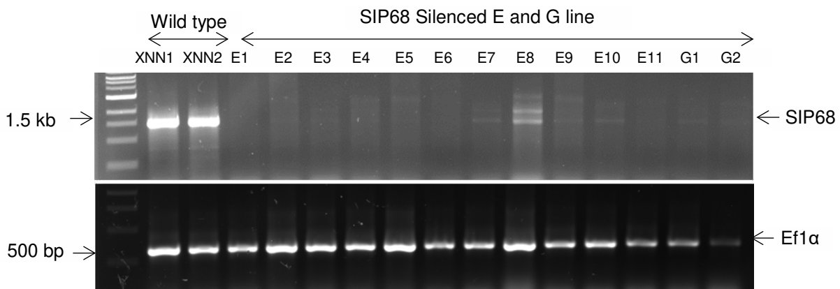
Figure 29: Screening of T2 RNAi Silenced #E and #G Lines. Ethidium bromide stained 0.8% and 1% agarose gel showing expression of SIP68 and Ef1α respectively. DNA ladder (1 kb) for SIP68 (~1491bp) and 100 bp ladder for Ef1α (~600) was used to compare a product size.
