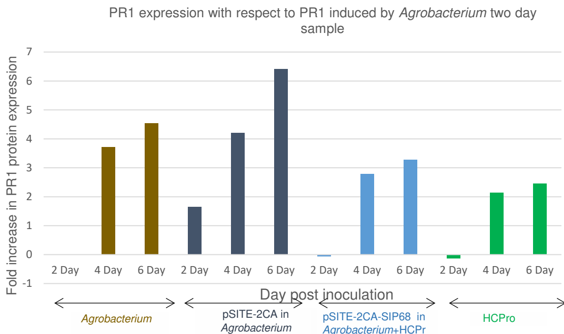
Figure 21: Densitometric Analysis of PR1 Expression at 2, 4 and 6 Days Post Infiltration of Agrobacterium , Agrobacterium +SIP68+ eGFP With and Without HCPPro, and HCPPro Only With Respect to Agrobacterium two-day Sample.
