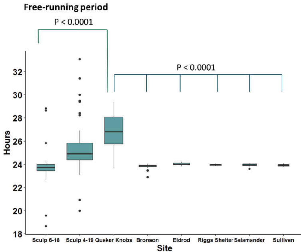
Figure 2.4: Box plot showing variation in free running periods between isolated caves. Both visits to Sculpture cave show a large amount of variation, Quaker Knobs cave individuals showed a longer than 24 h FRP (26.85 h.), and all the Indiana caves show FRPs close to 24 h. with little variation
