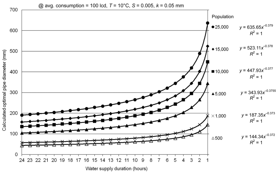
Figure 3. Water supply duration and calculated optimal pipe diameter for different population categories.
