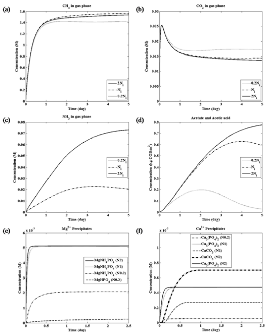
Figure 5.5 Effects of inorganic nitrogen on biogas in gas phase, substrate in liquid phase and precipitates in solid phase
