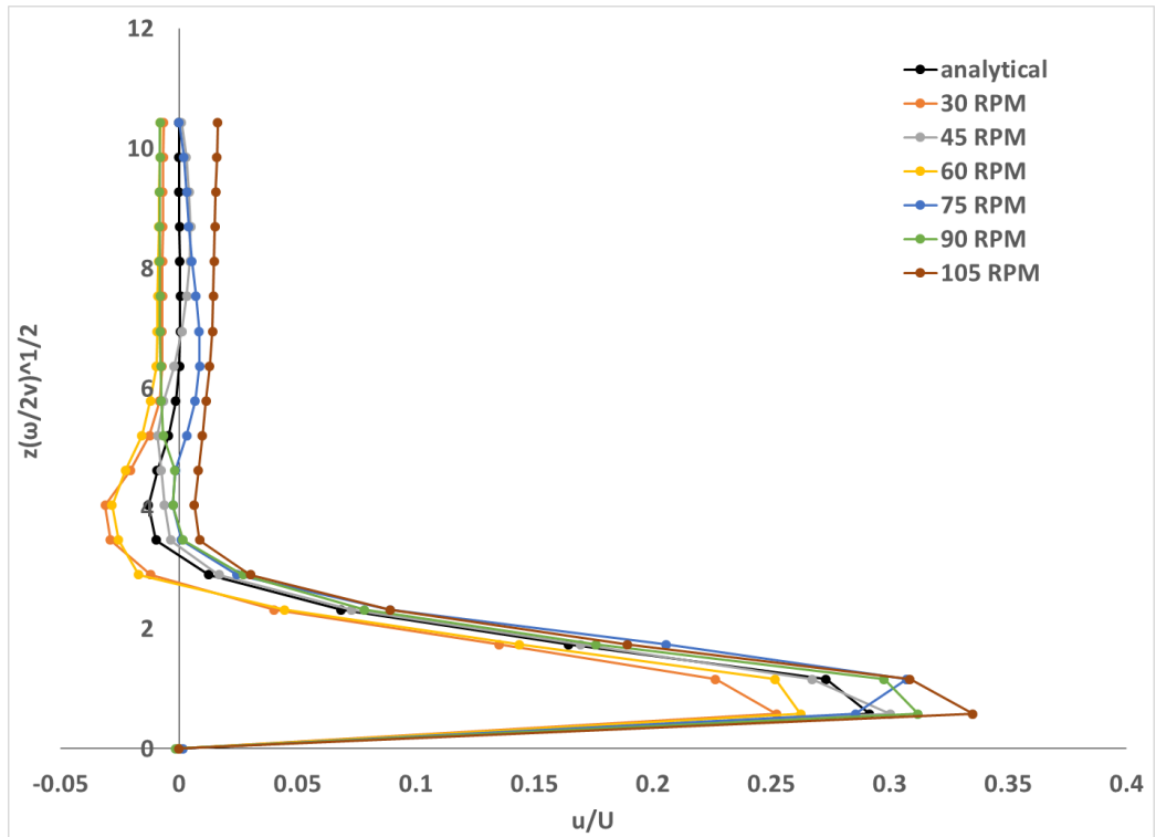
Figure 5.9. Comparison of analytical solution to computational u/U for each case from z(\omega/2v)^{1/2} of 0 to 10.44.
