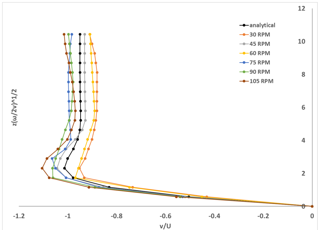
Figure 5.10. Comparison of analytical solution to computational v/U at for each case from z(\omega/2v)^{1/2} of 0 to 10.44.
