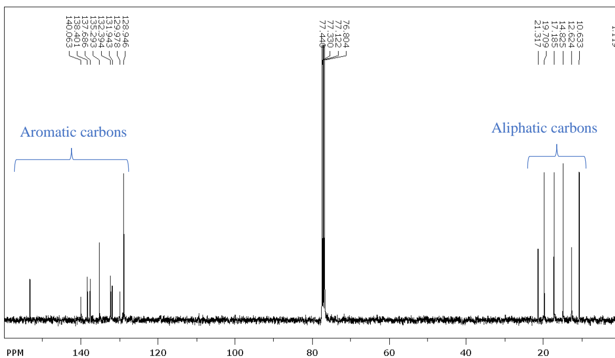
Figure 16: ^{13}\text{C} NMR of BODIPY analyzed in \text{CDCl}_3
