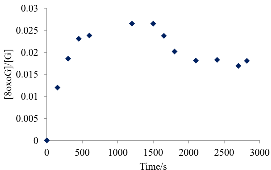
Figure 24. Accumulation of 8oxoG during DNA oxidation by SO_4^{\cdot-} produced by photolysis using the Hg(Xe) lamp of aqueous solution persulfate during indicated times. HPLC conditions were as previously indicated.
