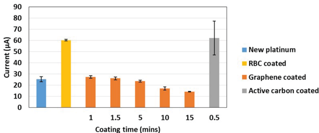
Fig 4.6 Comparison of graphene coated and active carbon coated electrode performance for current measurements of 60 vol% RBC in PBS at 100 V DC. Error bars represent 95 % confidence intervals.
