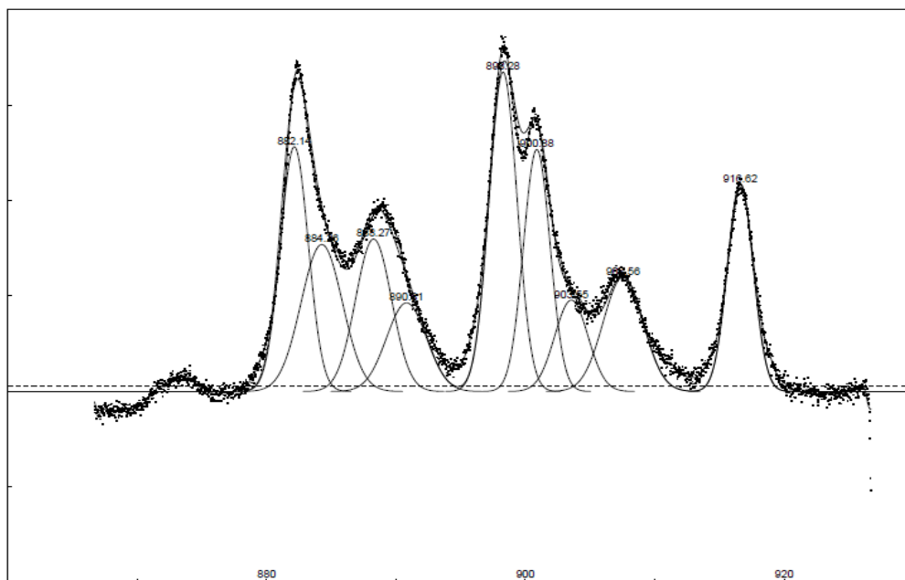
FIGURE A2-2 – CeO 2 nanoplates by NH 4 OH deconvoluted XPS spectrum
