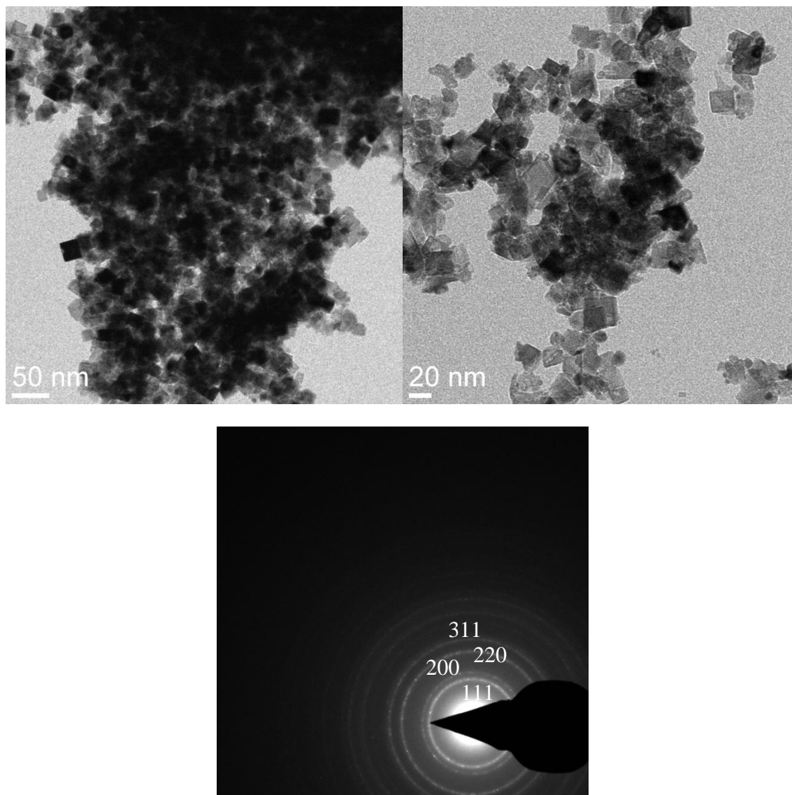
FIGURE 4.3 - TEM and SAED image of CeO 2 nanoplates by NH 4 OH at 100°C.
