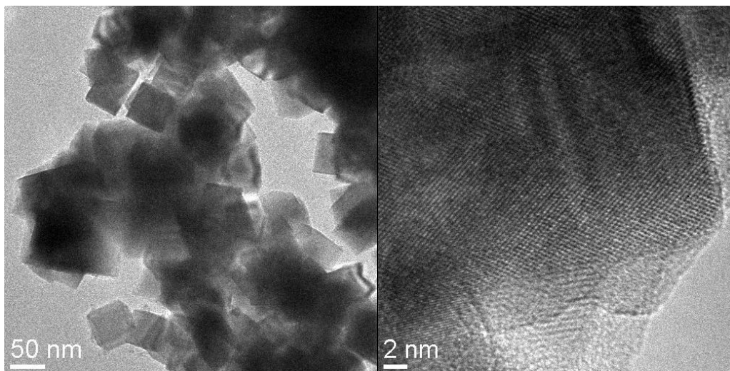
FIGURE 4.5 - TEM and HRTEM images of \text{CeO}_2 nanocubes with a C_{\text{NaOH}} = 9 \text{ M} at 180^\circ\text{C} .
