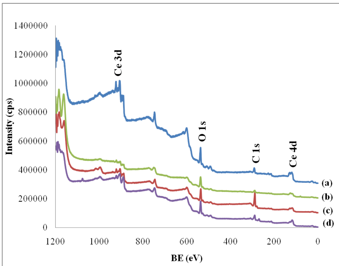
FIGURE 4.9 - XPS survey spectra of \text{CeO}_2 nanoplates by \text{H}_2\text{O}_2 (a), nanocubes (b), nanoplates by \text{NH}_4\text{OH} (c), and nanorods (d).
