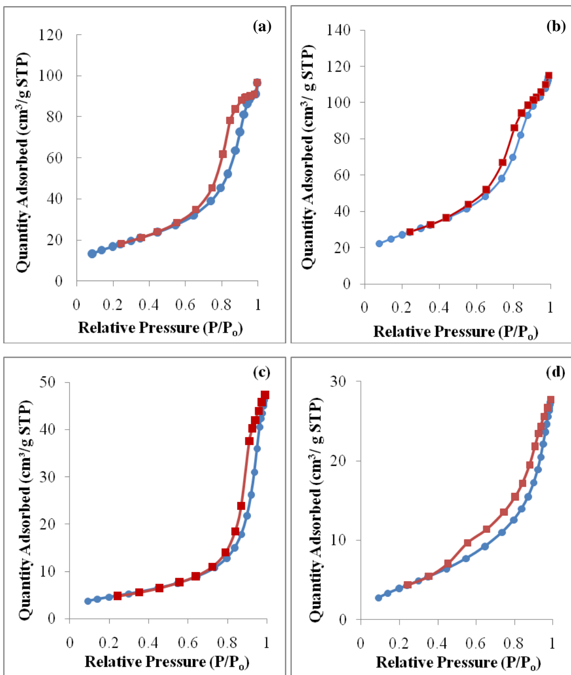
FIGURE 4.7 - Nitrogen adsorption-desorption isotherm pattern as synthesized of CeO_2 nanoplates using H_2O_2 (a), nanoplates using NH_4OH (b), nanocubes (c), and nanorods (d), (● adsorption, ■ desorption).
