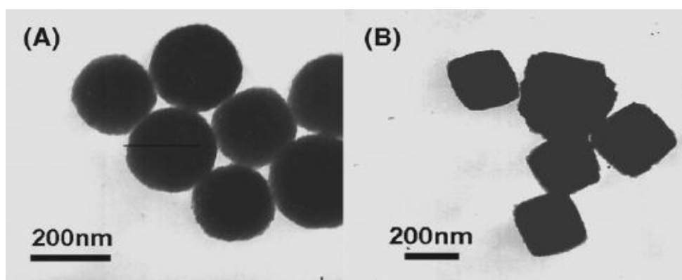
FIGURE 2.6 - TEM images of the products obtained by the utilization of varied cerium source: (A) (\text{NH}_4)_2\text{Ce}(\text{NO}_3)_6 ; (B) \text{CeCl}_3 \cdot 7\text{H}_2\text{O} (Yang, 2009).
