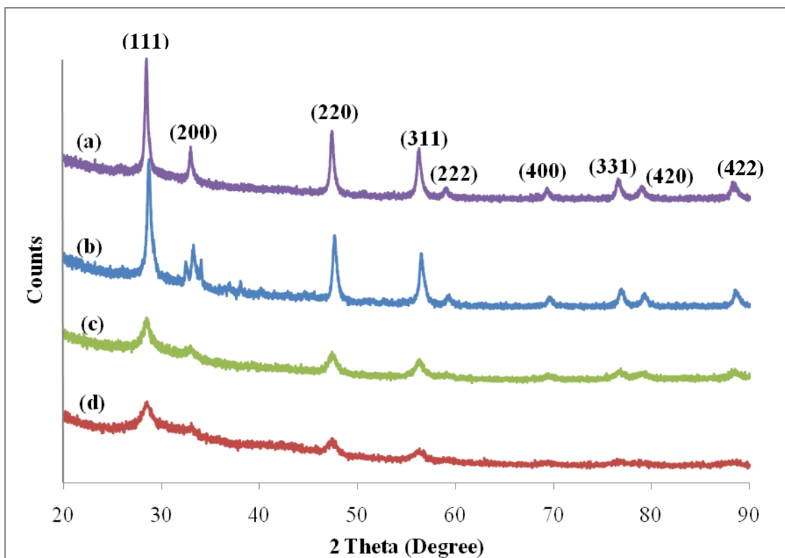
FIGURE 4.13 - XRD of \text{CeO}_2 nanoplates by \text{H}_2\text{O}_2 (a), nanocubes (b), nanoplates by \text{NH}_4\text{OH} (c), and nanorods (d).
