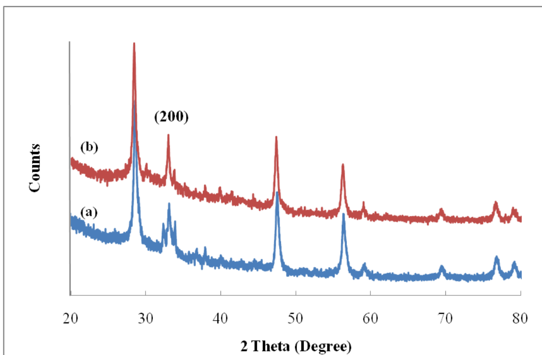
FIGURE 4.16 - XRD patterns of CeO 2 nanocubes ( C_{\text{NaOH}}=6\text{M} ) calcined at 100°C (a) and 400°C (b).
