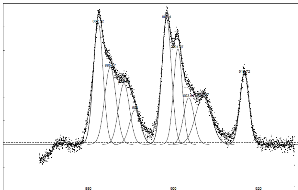
FIGURE A2-1 – CeO 2 nanoplates by H 2 O 2 deconvoluted XPS spectrum
