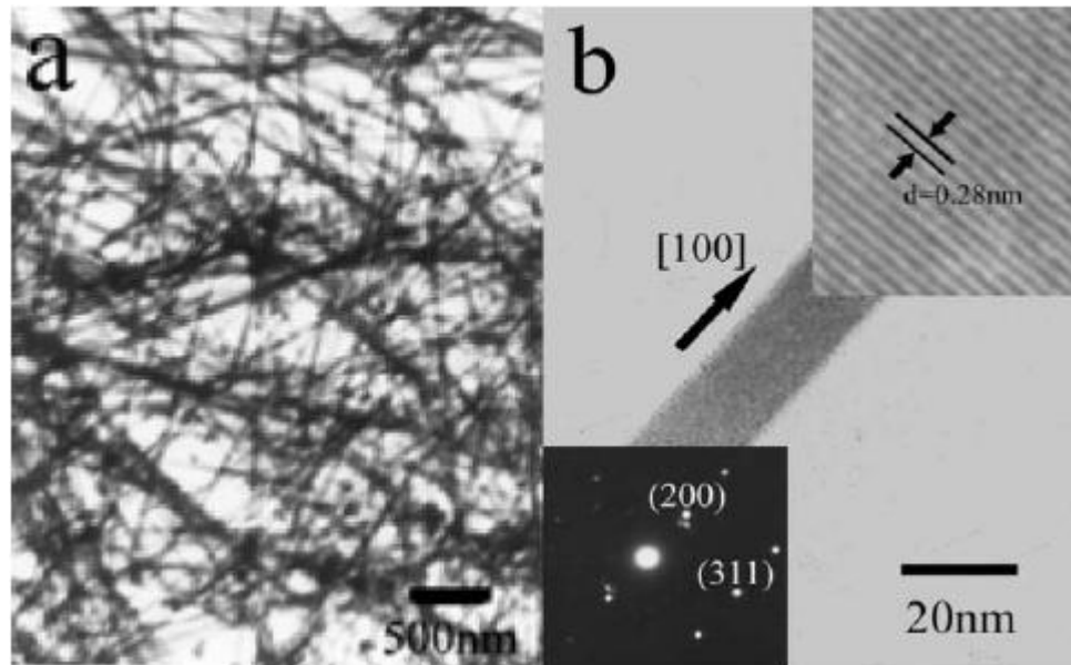
FIGURE 2. 3 - a) TEM image of \text{CeO}_2 nanowires, b) HRTEM image of individual \text{CeO}_2 nanowire (Tang,2005).
