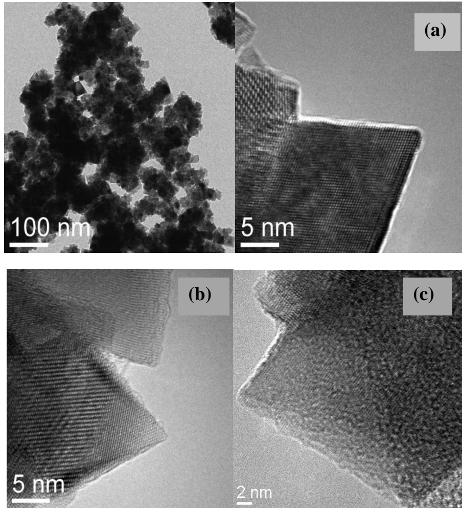
FIGURE 4.2 - TEM, HRTEM and SAED images of \text{CeO}_2 nanoplates by \text{H}_2\text{O}_2 synthesized at different temperatures (a) 180^\circ\text{C} for 24 hr, (b) 200^\circ\text{C} for 24 hr, and (c) 250^\circ\text{C} for 3h.
