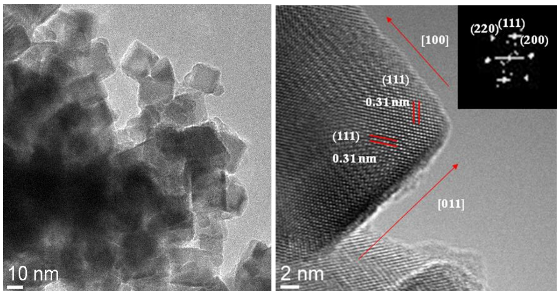
FIGURE 4.6 - TEM and HTERM images of \text{CeO}_2 nanocubes with a C_{\text{NaOH}} = 6 \text{ M} at 180^\circ\text{C} .
