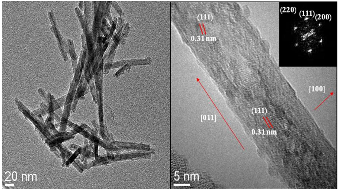
FIGURE 4.4- TEM and HRTEM images of \text{CeO}_2 nanorods with a C_{\text{NaOH}} = 9 \text{ M} at 100^\circ\text{C} .
