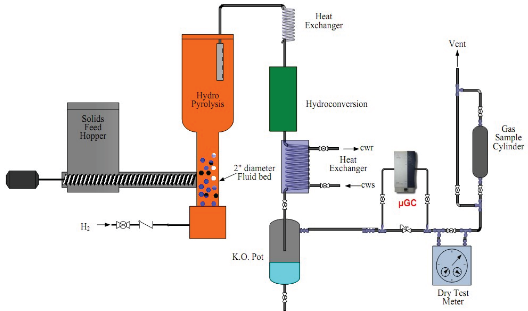
Figure 7.8 More detailed Simplified flow diagram of GTI IH 2 process. (Diagram reference from extended abstract 2009 AIChE by Terry Marker, Larry Felix and Martin Linck from GTI)
