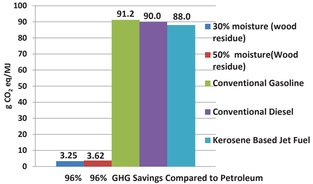
Figure 6.13 Results of IH 2 fuel for forest feedstock GHG emissions savings compared to petroleum fuels (no transport step to blending was included here-negligible effect).
