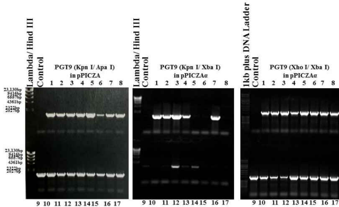
Figure 24. PCR Screen Results of Selected E.coli Colonies Transformed with Modified PGT 9 in pPICZA and pPICZA \alpha Vectors. Clone specific primers used for each modification were used in the PCR screens. Ligation into pPICZA and pPICZA \alpha as well as transformation into E. coli were successful.
