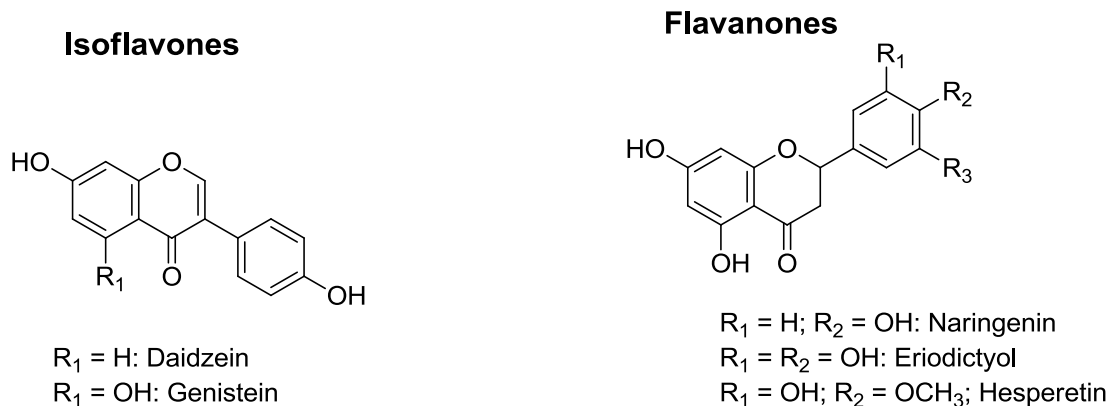
Figure 3. Flavonoids
