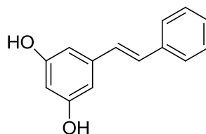
Pinosylvin
