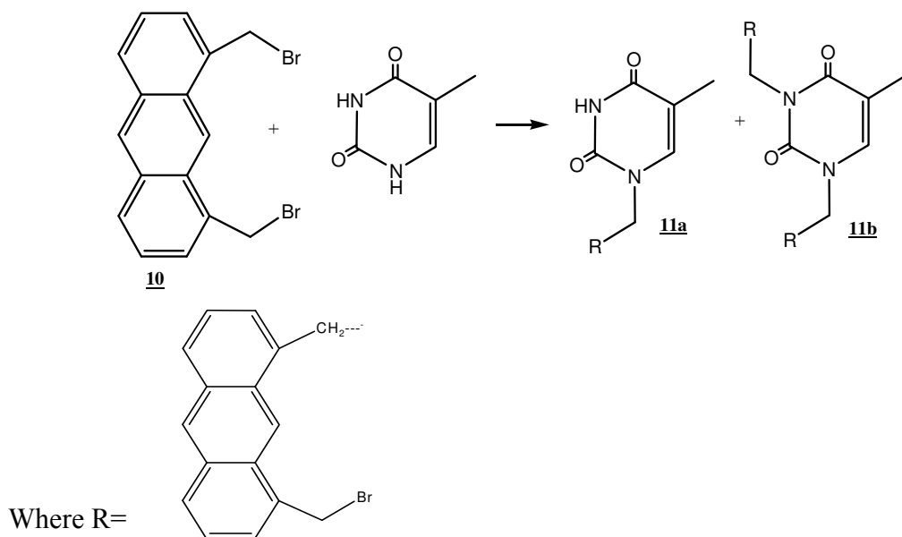
Scheme 16. Reaction of 1,8-Bisbromomethylanthracene with Thymine
