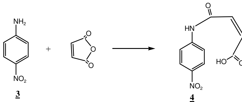
Scheme 12. Reaction p-Nitroaniline with Maleic anhydride
