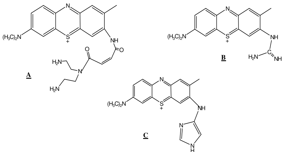
Figure 10. Nuclease Models Based on Toluidne Blue O
