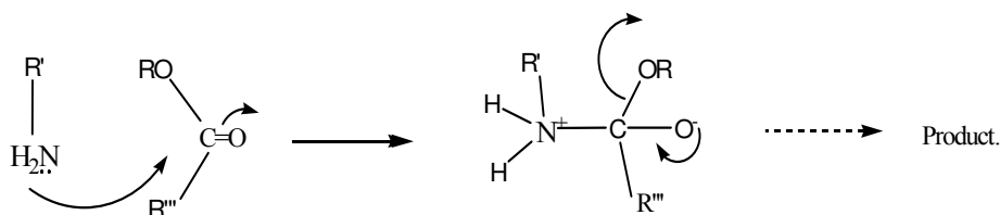
Scheme 8. Illustration of Alkylation (or Acylation) of a 1° Amine
