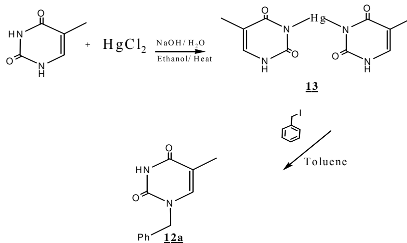
Scheme 17. Synthesis of Dithyminylmercury and its Reaction with Benzyl Iodide
