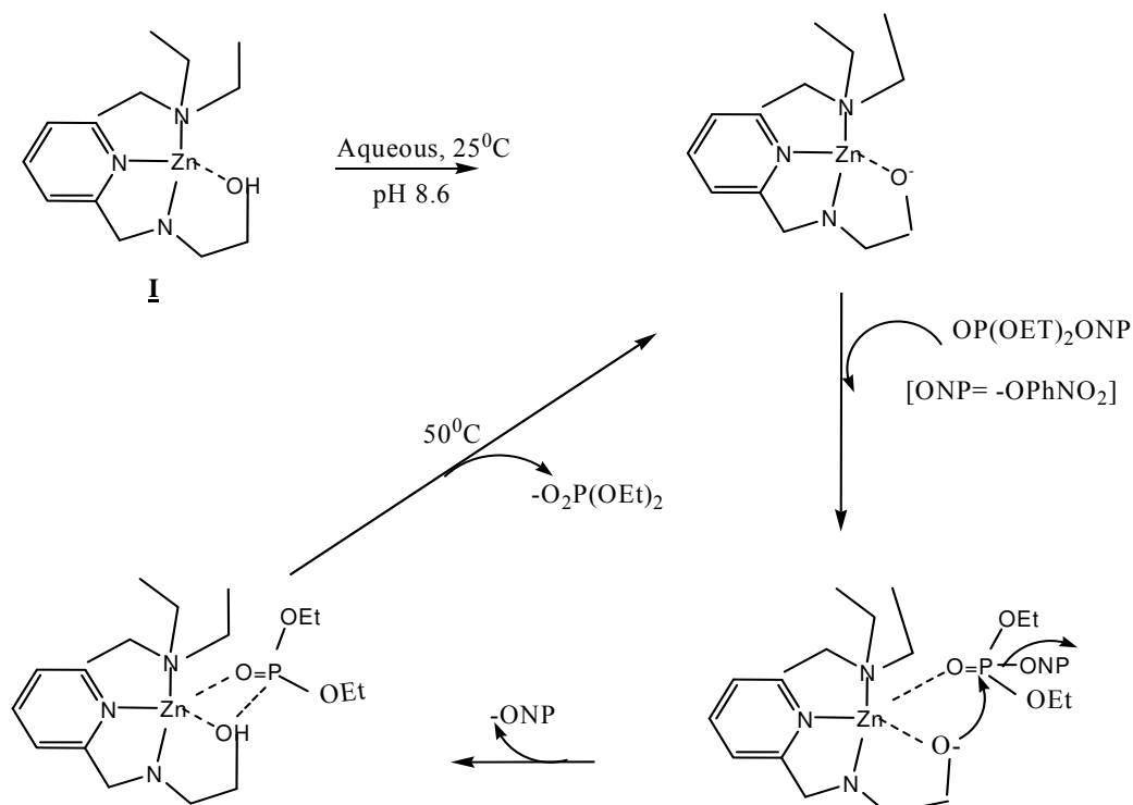
Scheme 5. Proposed Mechanism of Model I
