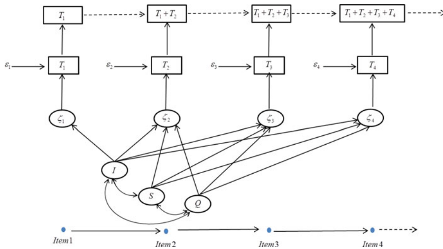
Figure 2. The lognormal random quadratic variable speed model. I = the random intercept; S = the growth rate; Q = the quadratic time component; T = the response time.
