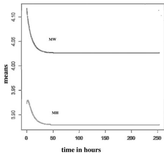
Figure 5. Mean development of MH and MW across time in terms of hours from measurement start, computed as e^{A(t-t_0)}E[\mathbf{x}(t_0)] + \mathbf{A}^{-1}[e^{A(t-t_0)} - \mathbf{I}]\mathbf{b} .
