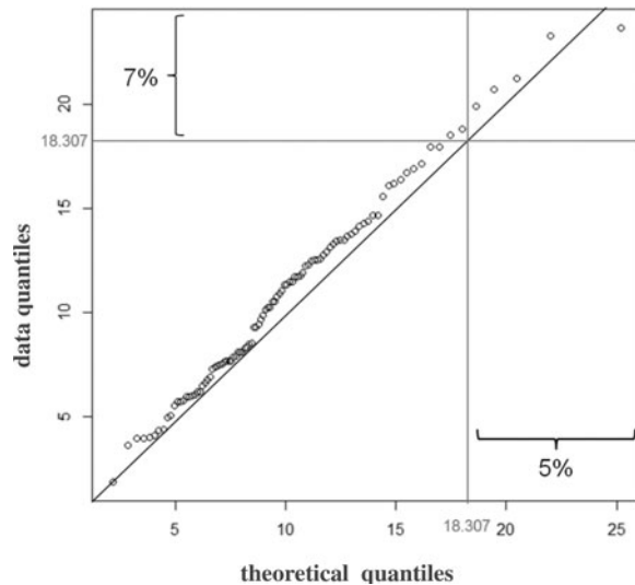
Figure 1. Q-Q plot for the 100 \chi^2 -values resulting from the subject-group-reproducibility tests in which 100 subjects, generated from the same model, were individually compared to each sample of remaining subjects.
