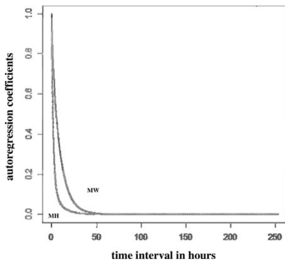
Figure 3. Autoregressive effects of mood at work (MW) and mood at home (MH) over intervals in terms of hours, computed as the diagonal elements of matrix exponential e^{A\Delta t} .
