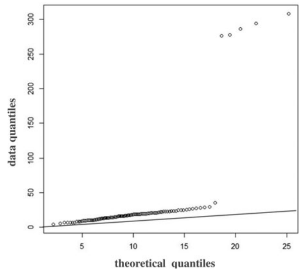
Figure 2. Q-Q plot for the 100 \chi^2 -values resulting from the subject-group-reproducibility tests on 100 subjects, of whom 95 were generated by one model and 5 others by a different model.
