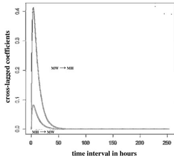
Figure 4. Cross-lagged effects of MW on MH (MW \rightarrow MH) and MH on MW (MH \rightarrow MW) over intervals in terms of hours, computed as the off-diagonal elements of matrix exponential e^{A\Delta t} .
