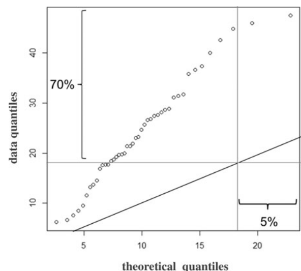
Figure 7. Q-Q plot for 44 \chi^2 -values resulting from the subject-group-reproducibility tests in which the 55 women in the real life example were individually compared to each sample of 54 remaining subjects; 11 \chi^2 -values for analyses with lacking standard errors were omitted.
