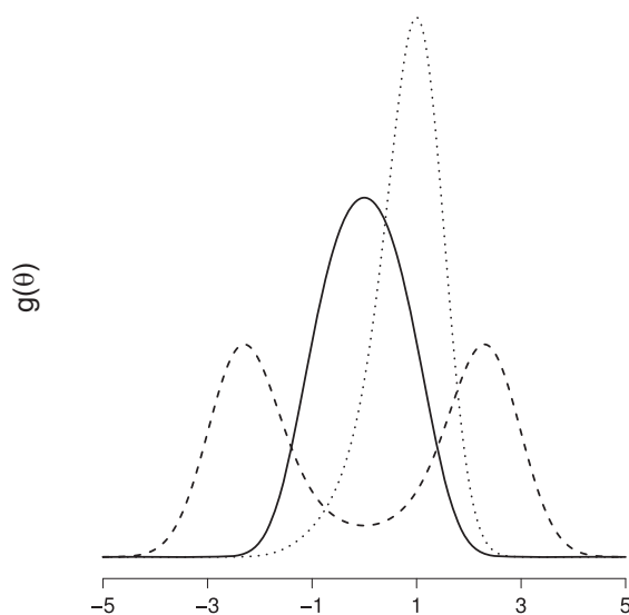
Figure 7. Some instances of the structural model g(\theta) for the n = 6 variable network. The solid line refers to the distribution with \sigma = 0.1 and the \mu_i equally spaced between -1 and +1 . The dashed line refers to the distribution with \sigma = 0.2 and the \mu_i equally spaced between -1 and +1 . The dotted line refers to the distribution with \sigma = 0.1 and the \mu_i equally spaced between -0.2 and +1 .
