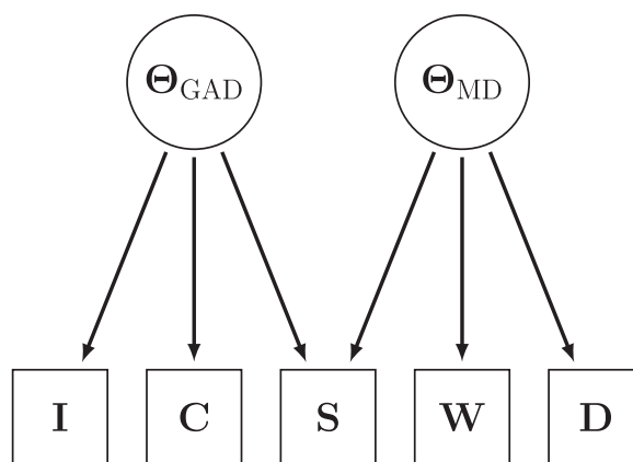
Figure 4. A common cause representation of the manifest relations between GAD and MD symptoms in Figure 3.
