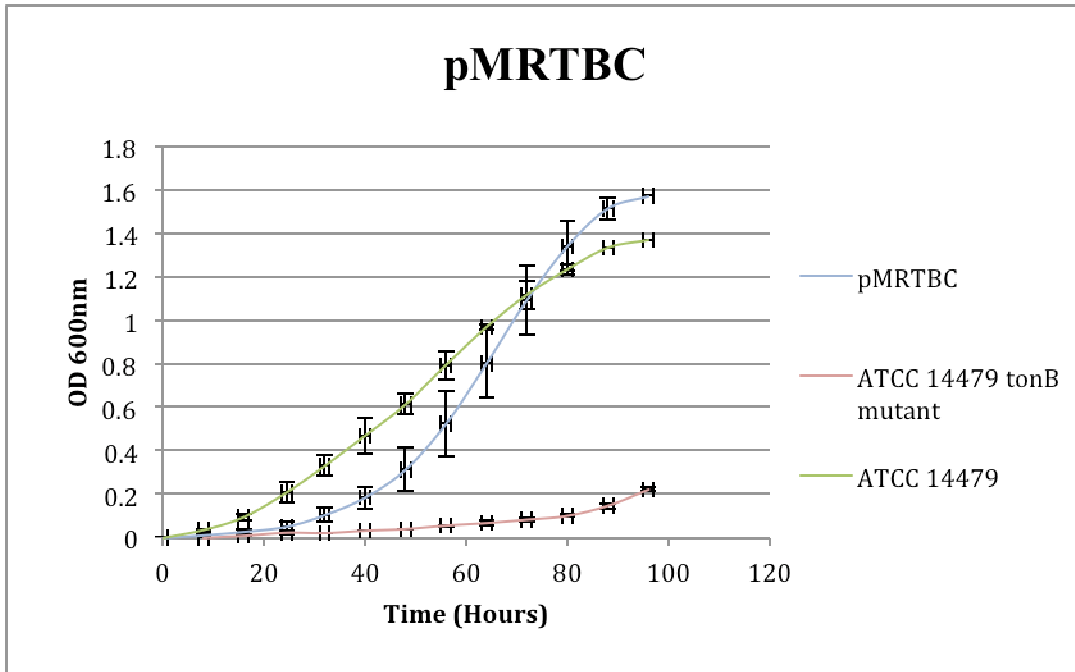
Figure 18. Growth Curve of wild type ATCC 14479, RL \Delta TB harboring pMRTBC, and mutant RL \Delta TB in low iron media. Strains were grown in MMW Na10Pg50 supplemented with 0.25mM 2,2 dipyridyl and 0.25mM FeCl 3 .
