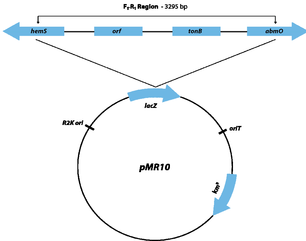
Figure 2. pMR10. Diagram of pMR10
