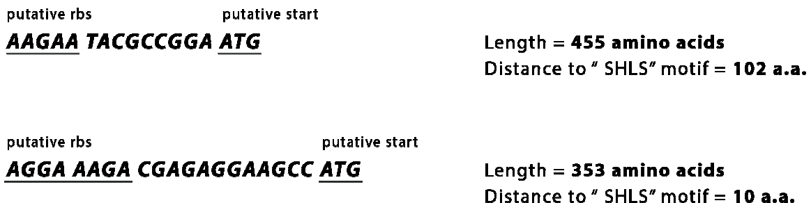
Figure 21. Putative RBS and translational start sites of pMRTP1 and pMRTP2.
