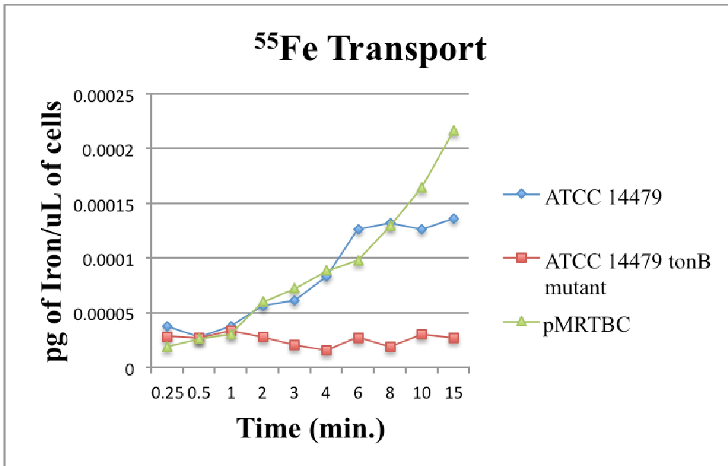
Figure 19. 55 Fe-Vicibactin Time-Dependent Transport assay of wild type ATCC 14479, RL \Delta TB harboring pMRTBC, and mutant RL \Delta TB. Wild type ATCC 14479 (blue), RL \Delta TB harboring pMRTBC (green), and mutant RL \Delta TB (red).
