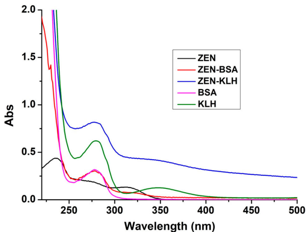
Figure 3. The UV spectra characterization for ZEN-KLH, ZEN-BSA, ZEN, KLH, and BSA.
