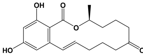
Figure 1. Chemical structure of zearalenone.
