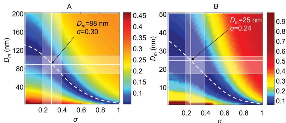
Figure 3. Colour maps of the maximum likelihood estimators \chi^2 value as a function of the distribution width \sigma , and the median diameter D_m for location A: HAB = 38 nm and r = 2.2 mm and B: HAB = 42 mm and r = 0 mm. The best fit value is shown in each figure.
