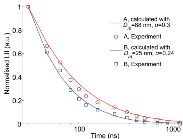
Figure 6. Normalised LII signal at 400 nm as a function of time at flame locations A and B. The best fit of experimental LII signals at the two different locations was found by 2-parameter fitting.
