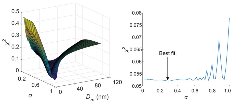
Figure 4. Left: 3D plot of \chi^2 for location A; right: value of the minimised \chi^2 along the valley.
