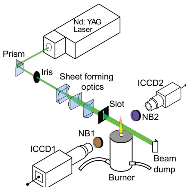
Figure 1. Schematic of 2D-2C-TiRe-LII measurement set-up (B1: 400 \pm 5 nm band filter; NB2: 450 \pm 5 nm band filter).
