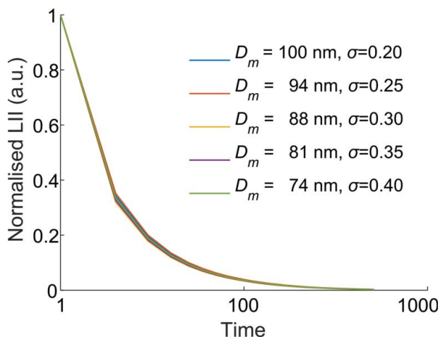
Figure 5. Reconstructed LII signal with selected (D_m, \sigma) pairs in the valley of minimising values.
