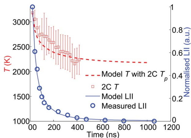
Figure 7. Measured LII signal at 400 nm (blue symbols, right scale), model LII using minimum error method for mean diameter and its distribution, as well as 2C method for peak temperature (solid blue line). Measured particle temperature T (red squares, left scale) using the two colour method; modelled T starting from the 2C peak measurement T_p = 3181 K.
