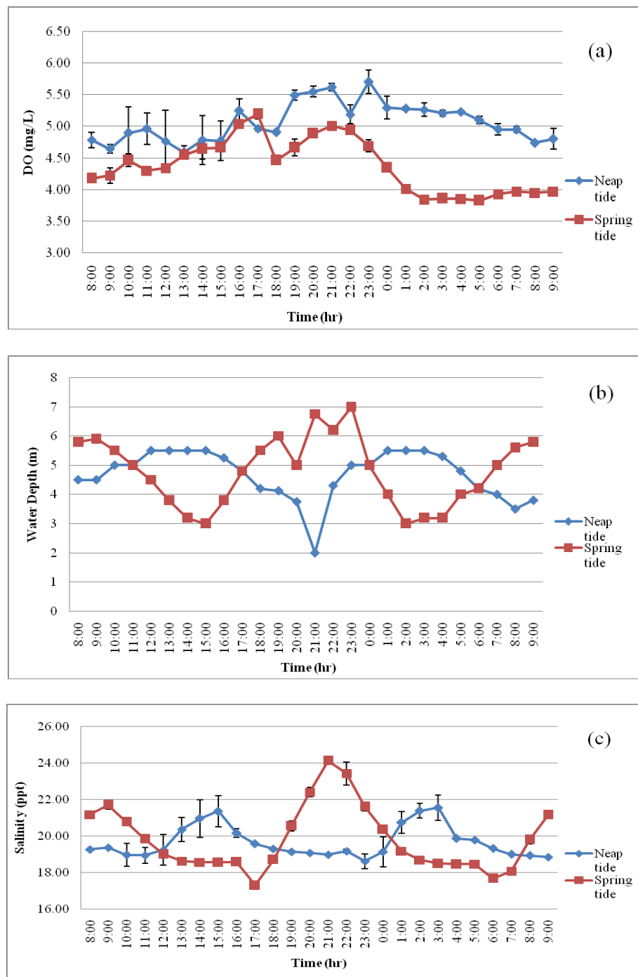
Figure 2 Dissolved oxygen, water depth, and salinity data from the temporal studies on June 14 th (neap tide) and June 22 nd (spring tide), 2005, in the Skidaway River Estuary, GA DO and salinity values are depth-averaged. Error = 1 SD.
