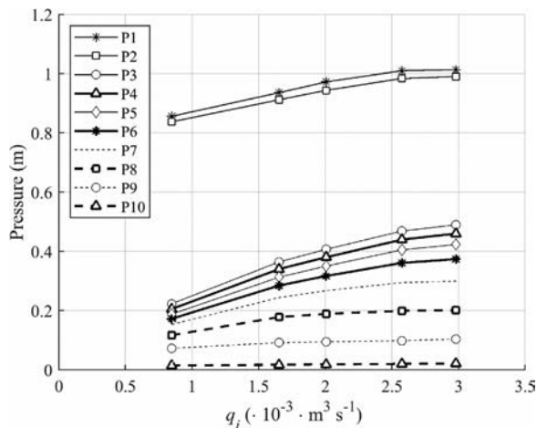
Figure 8. Pressure measurements for Test 1 from Table 1 (Figure adopted from Ravindra 2020).
