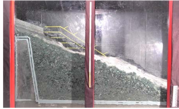
Figure 11. Image of model without toe during breach.
