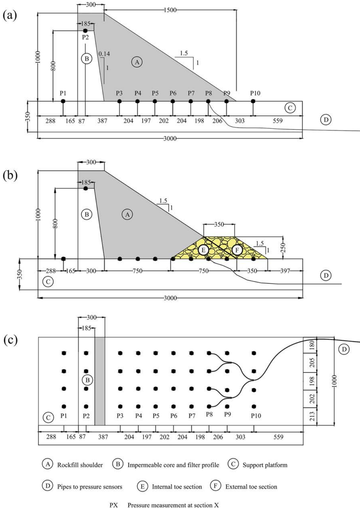
Figure 3. Depictions of the experimental setup with (a) sectional view of the rockfill dam model, (b) details regarding the disparate toe configurations and (c) planar view of the horizontal platform. (Figure adopted from Ravindra 2020).
