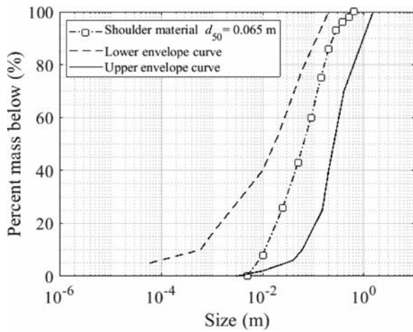
Figure 6. #Grain size distribution enveloping curves (scaled 1:10) from dam database and for chosen shoulder material (unscaled).
