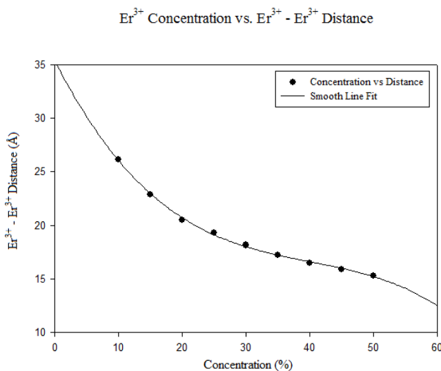
Fig 4.2: Graph depicting how the Er 3+ separation distance changes with increasing concentration, according to Eq 2.11.
