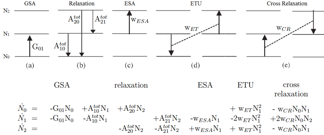
Fig. 2.2: The five main processes of concern in the thesis, along with their rate equations. The processes are (a) ground state absorption, (b) relaxation, (c) excited state up-conversion, (d) energy transfer up-conversion, and (e) cross relaxation. Note the superscript tot on the A coefficient, this is defined as the sum of both radiative and non-radiative relaxation processes.
