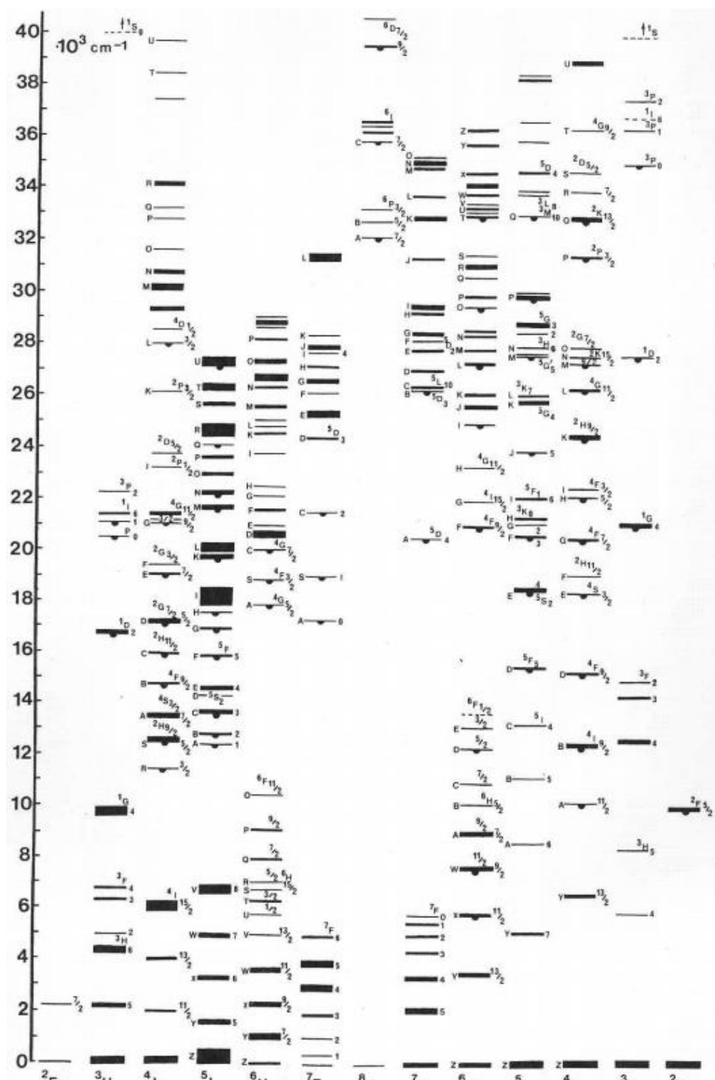
Fig 1.1: Dieke diagram showing the energy levels of the trivalent rare-earth ions in the host crystal \text{LaCl}_3 , compiled by Dieke in 1963 [18].
