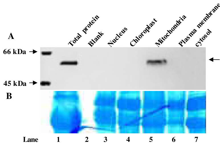
Figure 79: Western blot analysis of subcellular fractions. Panel A, western blot analysis using anti-c-myc antibody. Panel B, coomassie blue stain of the membrane, which serves as a loading control. Lane# 1; total protein and lanes# 2-7; blank, nucleus, chloroplast, mitochondria, plasma membrane, and cytosol fractions respectively. Arrow indicates the detection of SIP-428 expression.
