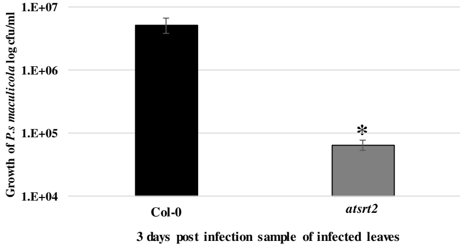
Figure 23: Bacterial growth assay in Arabidopsis wild-type Col-0 and atsrt2 . Figure shows CFU of Psm in atsrt2 mutant and the wild-type Col-0 at 3 days post infection (DPI). Student t test was used for statistical analysis ( P < 0.05 ) with multiple samples.
