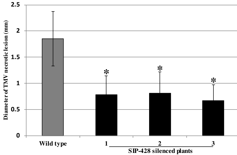
Figure 48: Systemic acquired resistance in SIP-428 silenced lines. Bar diagram shows the average diameter of TMV lesion size with standard deviation in wild-type (gray), and SIP-428 silenced plants (black). Three independent SIP-428 silenced lines (1, 2, and 3) and multiple wild-type controls were used (P < 0.05).
