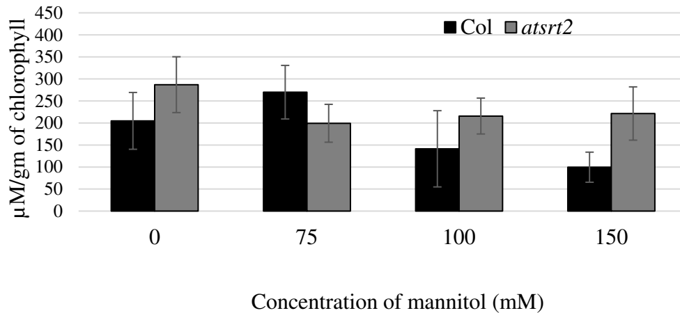
Figure 28: Effect of osmotic stress on chlorophyll content in wild-type (Col-0) and atsrt2 mutant plants. Bar diagram represent the average of chlorophyll content with Standard deviation for Col-0 (black) and atsrt2 (gray) ( P < 0.05 ).
