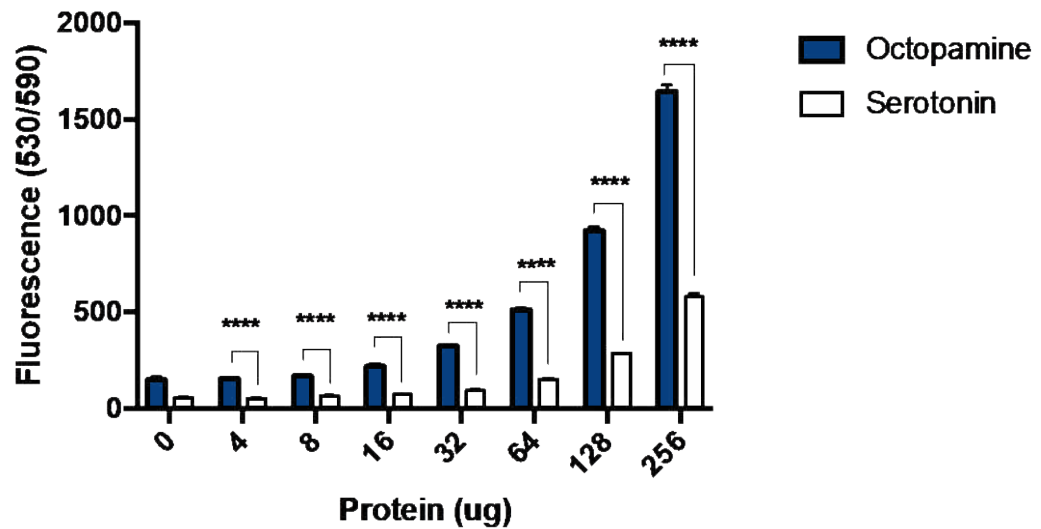
Figure 4.5. A) Protein concentration curve of detection of MAO activity from protein samples collected at 13 hours and 19hours. Data are mean \pm SD of triplicate wells. B) Protein concentration curve of detection of MAO activity of octopamine and serotonin as substrates (0.1mM). Data are mean \pm SD of triplicate wells. (*, p <0.05; **, p <0.01; ***, p <0.001; ****, p <0.0001)
