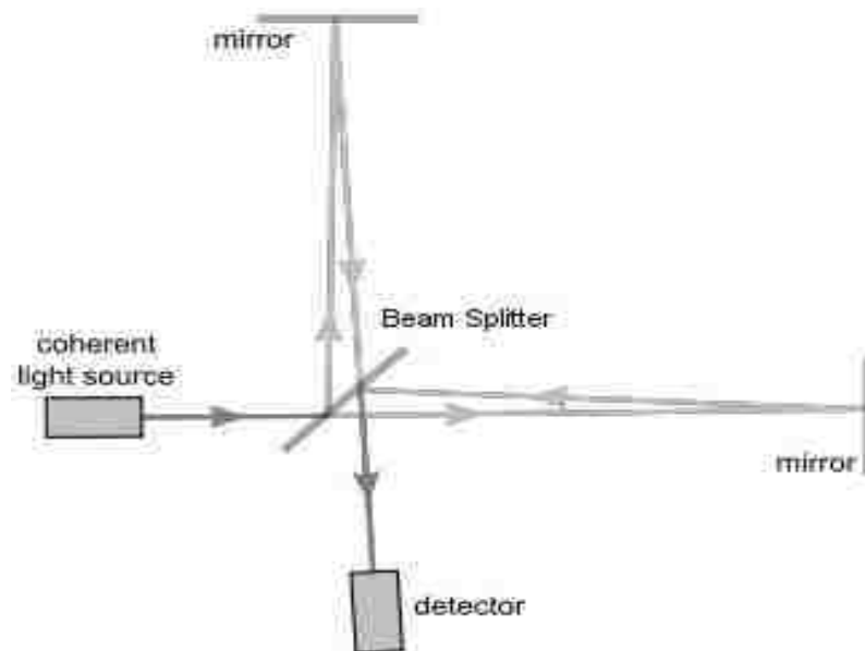
Figure 1.1 Michelson Interferometer
