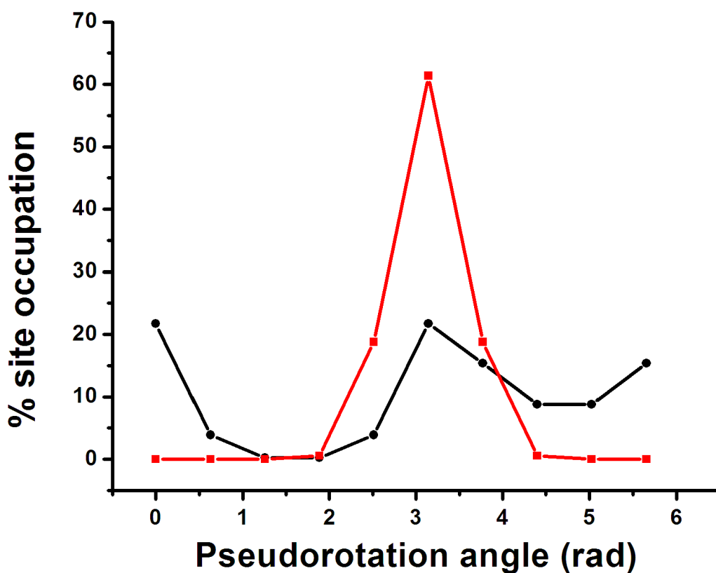
Figure 2.8. Overlay of the site populations for the trajectories of the potential energy used in the best fit simulations (red) for U:A and T:A compared to an arbitrary unequal double (Figure 2.2(B)) well of barrier heights 5 k_B T and 1 k_B T (black). The symbols represent the ten sites along the discretized trajectory. specific details discussed in the main text.
