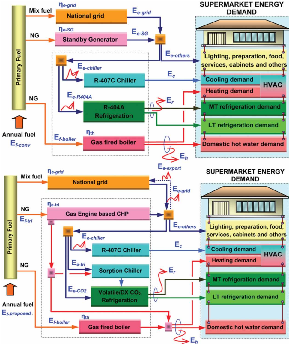
Figure 14. Energy flow diagram of a case-study supermarket with conventional and proposed energy system. Source: Suamir and Tassou (2013).
