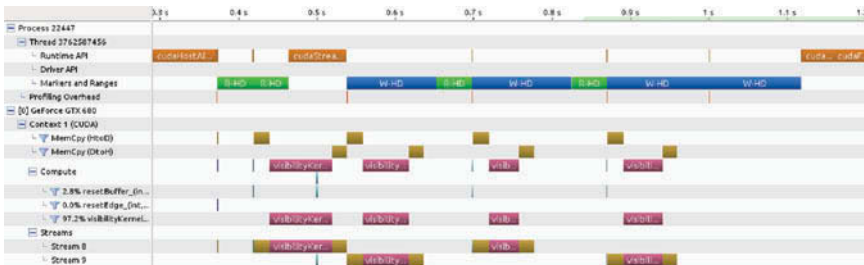
Figure 18. The Timeline View from NVIDIA visual profiler for concrete viewshed analysis for data divided into the four segments. In the Runtime API row are cudaHostAlloc call (left) and cudaFreeHost call (right). In the Markers and Ranges row are CPU reading from and writing to HD routines (R-HD and W-HD). In the Stream 8 and the Stream 9 rows are GPU cudaMemCpy and main viewshed kernel routines.
