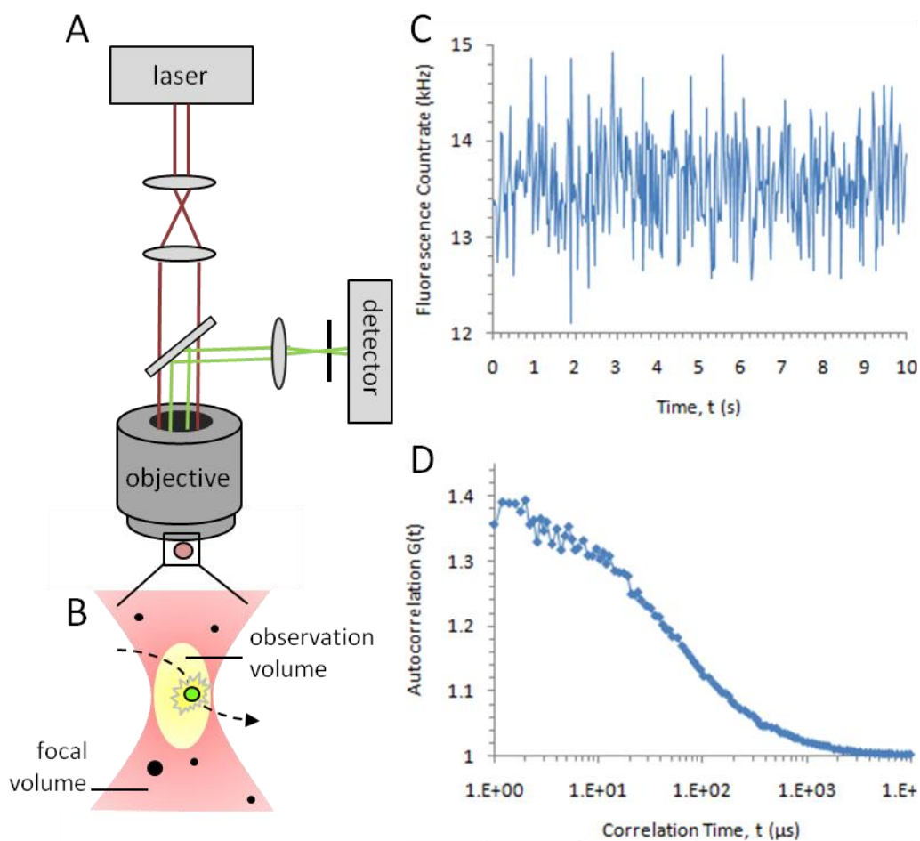
Figure 2.2. Schematic of FCS instrumental setup (A) and the confocal volume created (B). Fluorescent fluctuations (C) are recorded as fluorophores diffuse through the confocal volume and are used to calculate an autocorrelation curve (D).
