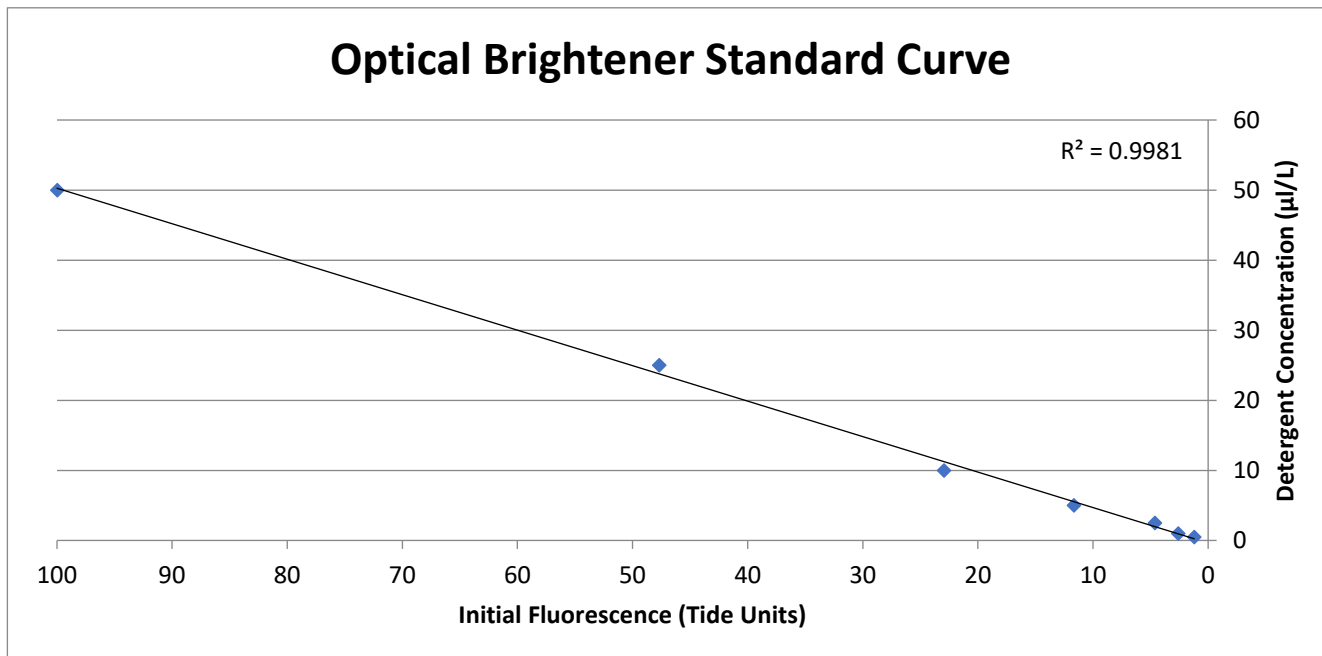
Figure 5. Initial fluorescence was measured for known concentrations of Tide 2X Original Scent detergent. From this graph, the amount of detergent in a water sample could be determined based on the initial fluorescence of a sample.
