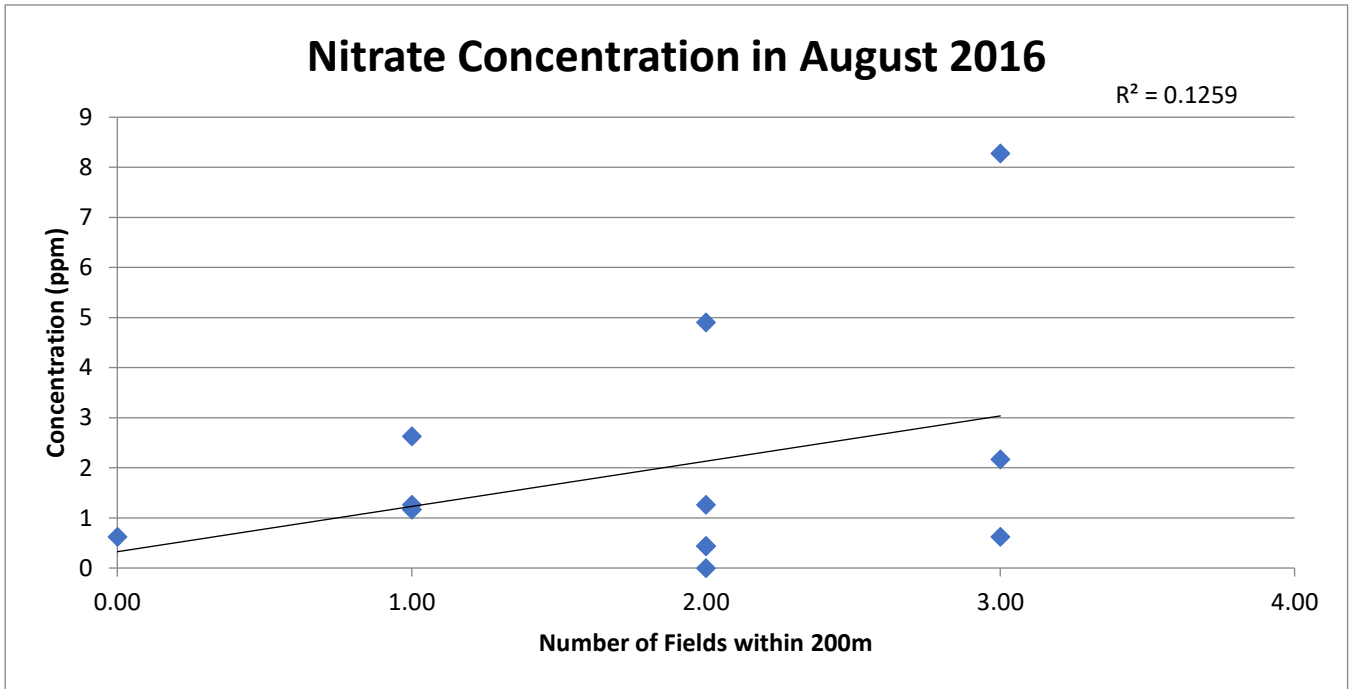
Figure 7. Number of septic fields within 200m of the sample site were compared to the concentration of nitrate in each sample site. The R^2 is 12.5% and the p-value is 0.26.
