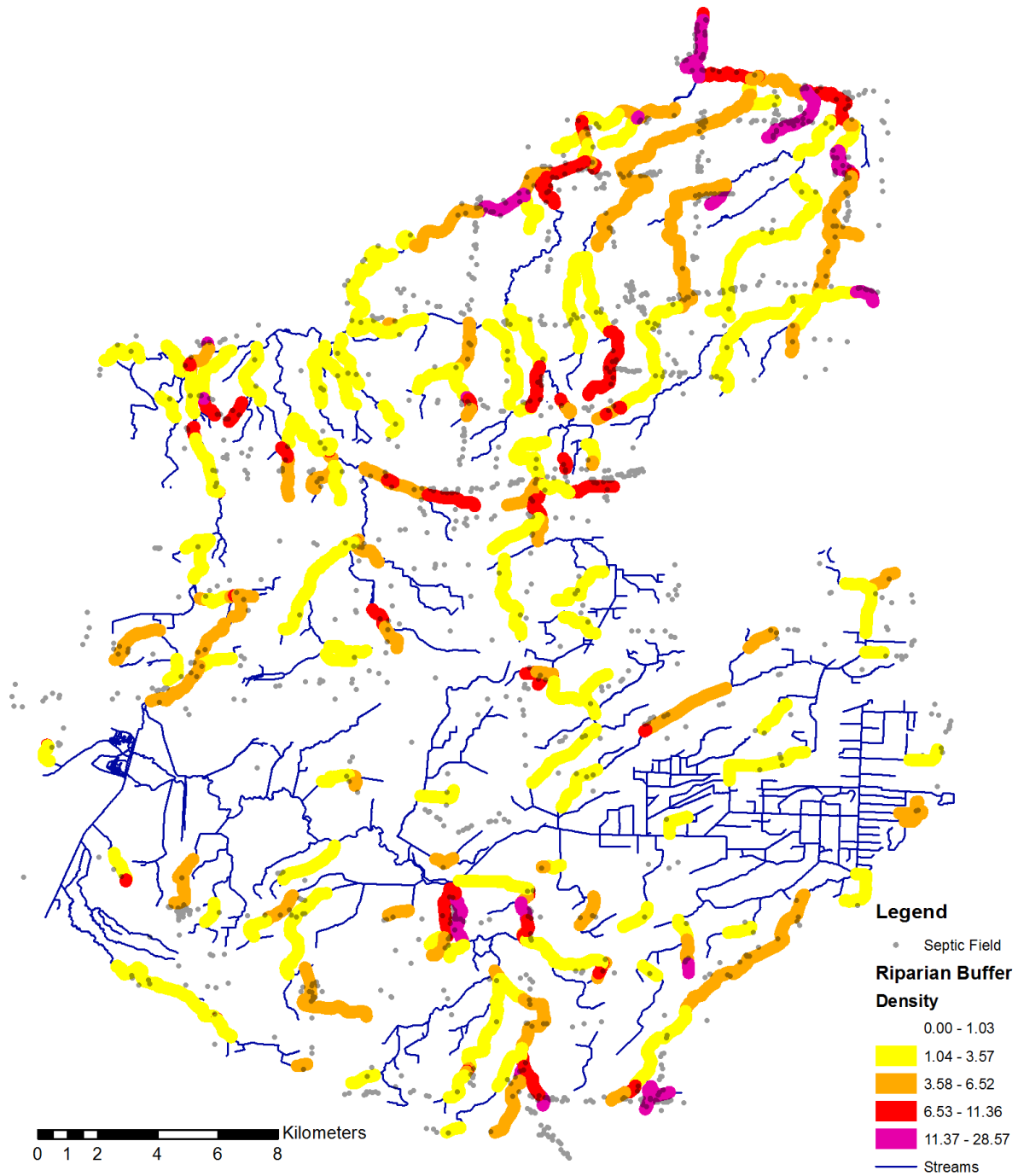
Figure 3. Septic field density within the 200m riparian corridor in the Oak Orchard watershed. Density is expressed as numbers of septic fields per square kilometer. Areas of stream segments with high densities are of interest because they may have greater septic inputs.
