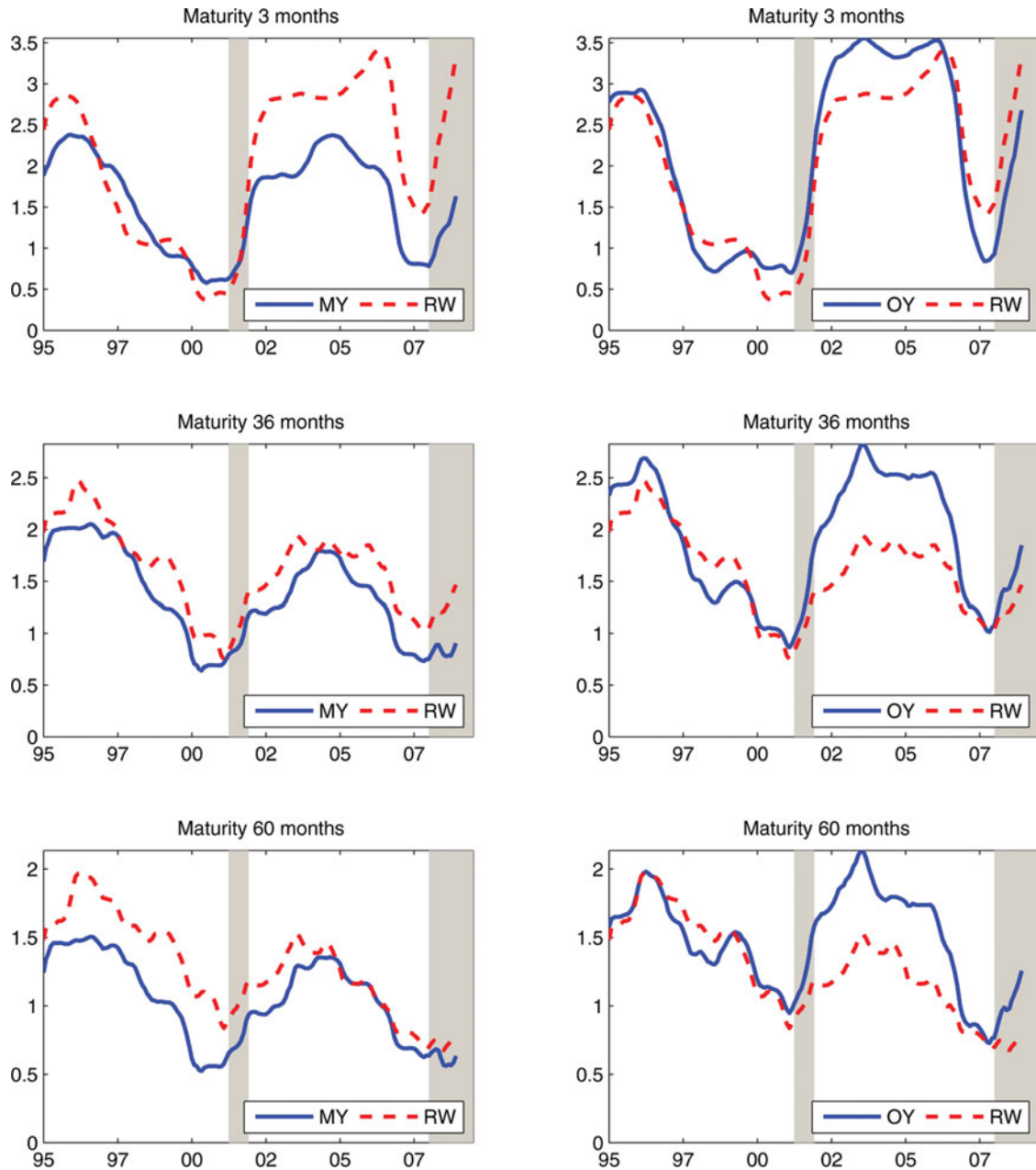
Figure 4. 12-months ahead smoothed squared forecast errors for yields. This figure displays the 5-years rolling 12-months ahead squared forecast error for the yields with 3, 36, and 60 months to maturity. The blue continuous line refers to the 5-years rolling squared forecast error of the macro-yields MY model (left plots) and of the only-yields OY model (right plots). The dashed red line refers to 5-years rolling squared forecast error of the random walk. The dates on the horizontal axis refer to the end of the rolling window period. The gray-shaded areas indicate the recessions as defined by the NBER.
