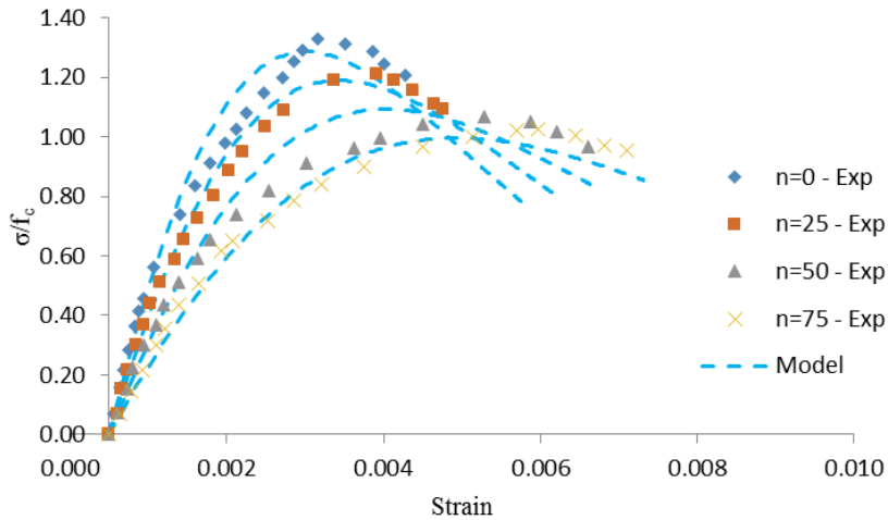
Figure 5.8. Stress-strain under biaxial compression ( \xi=0.5 ) after different CFT (Shang and Song, 2006)
