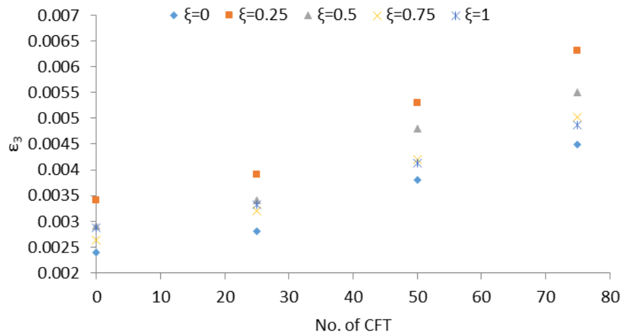
Figure 2.19. Ultimate strain versus number of CFT, data by (Shang and Song, 2006)
