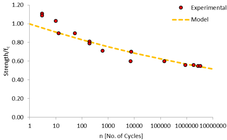
Figure 6.4. S-n curve for concrete under uniaxial cyclic loading, experimental data by (Yin and Hsu, 1995)
