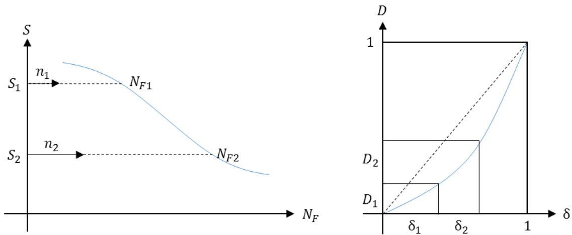
Figure 2.15. Illustration of the linear Palmgren-Miner law
