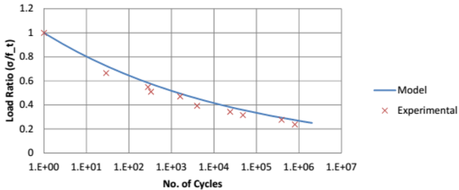
Figure 4.2. S-N curve for woven fabric composite under uniaxial fatigue loading, data by (Smith and Pascoe, 1989)
