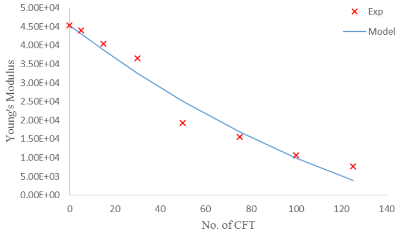
Figure 5.10. Modulus of elasticity versus number of CFT for uniaxial compression (Shang and Song, 2006)
