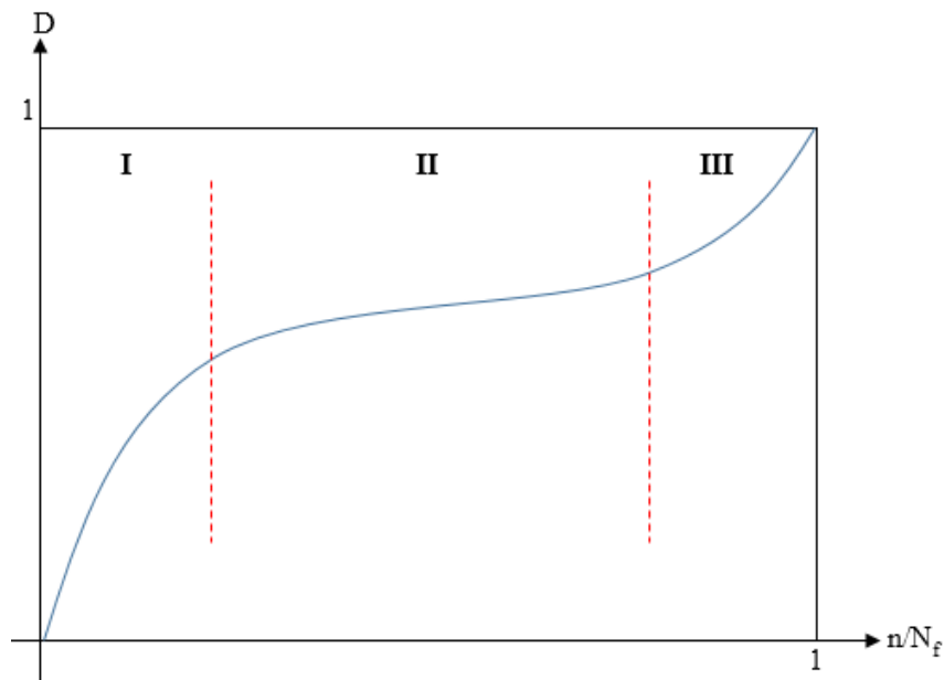
Figure 2.8. Damage accumulated versus fatigue life ratio
