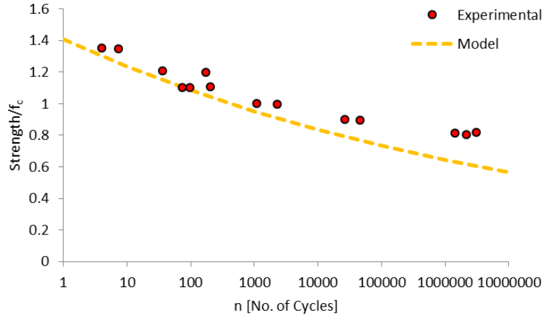
Figure 6.5. S-n curve for concrete under biaxial cyclic loading with stress ratio 0.5, experimental data by (Yin and Hsu, 1995)
