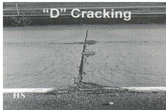
Figure 2.16. D-cracking in concrete pavement
