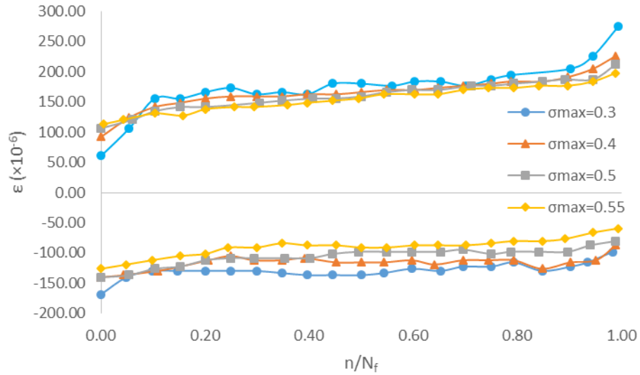
Figure 2.9. Strain versus fatigue life ratio, data by (Song et al. , 2005)
