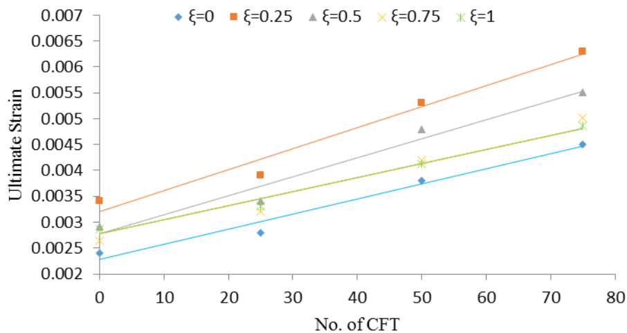
Figure 5.4. Influence of CFT on the principal \epsilon_3 under various stress ratios ( \xi=\sigma_1/\sigma_2 ) (Shang and Song, 2006)
